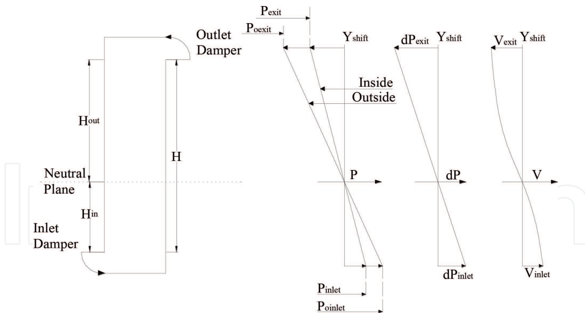
Figure 4. Air motion pattern in natural ventilation.
