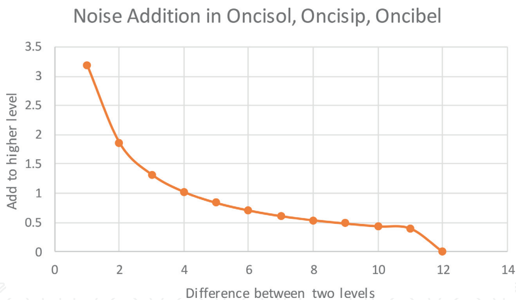
Figure 2. Noise addition.
