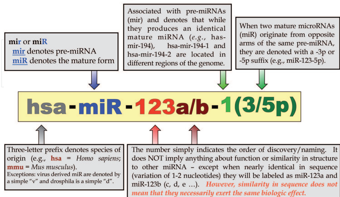
Figure 2. miRNA nomenclature explained. An important concept to understand is that the miRNA number (e.g., 123 as shown) has no relationship to function or structure. For example, “ hsa-miR-123 ” has no implied structural or functional similarity to “ hsa-miR-128 .” However, because of the highly conserved nature of miRNA, human “ hsa-miR-123 ” has very similar structure and function to murine “ mmu-miR-123 .”
