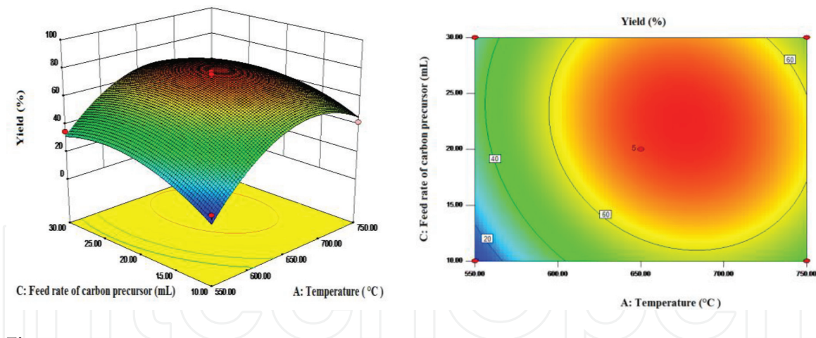
Figure 11. Response surface and contour plots for the yield of MWNTs as the function of temperature and feed rate of precursor.
