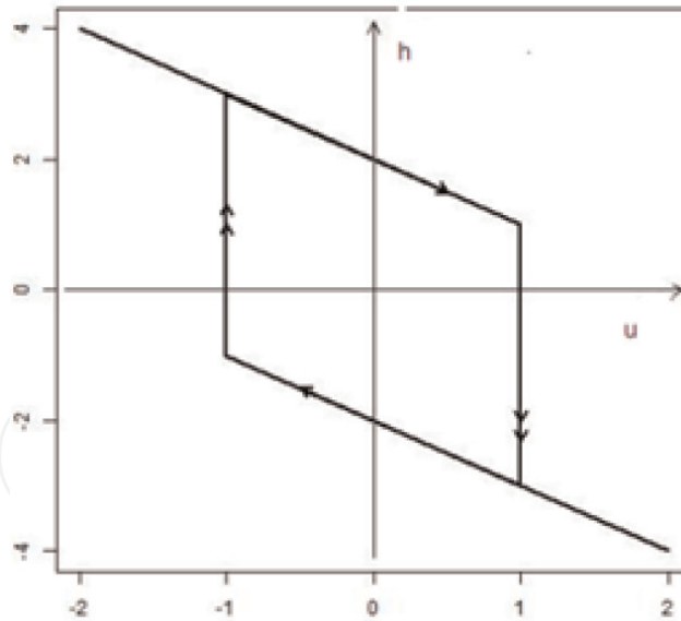
Figure 8. Relaxation oscillator defined by (15).
