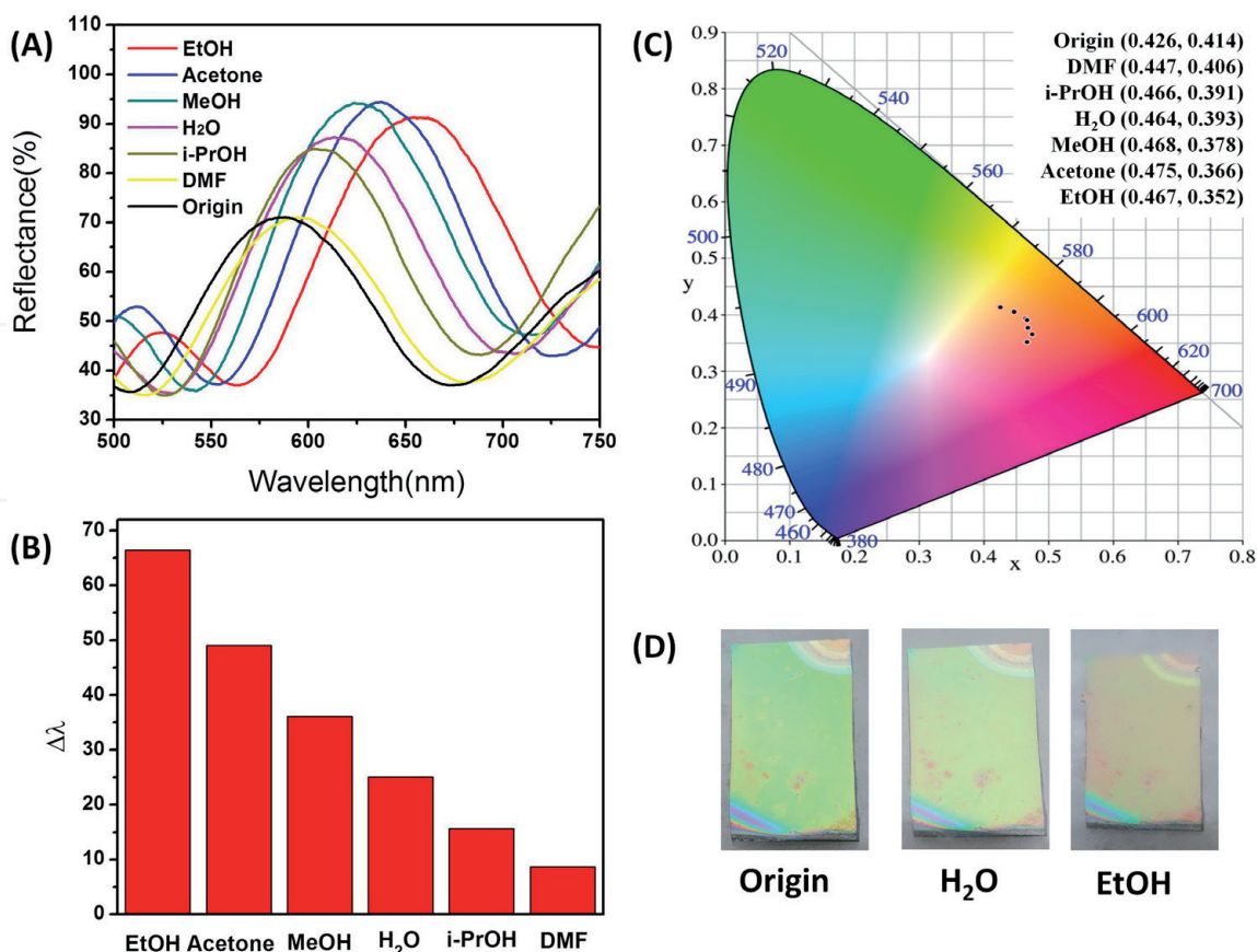
Figure 5. (A) Reflection spectra, (B) shift of the photonic stop band, (C) chromaticity coordinates, and (D) typical images of the \text{NH}_2\text{-MIL-88B}/\text{TiO}_2 1DPCs upon exposure to various organic vapors. Reproduced from Ref. [22] with permission from The Royal Society of Chemistry.
