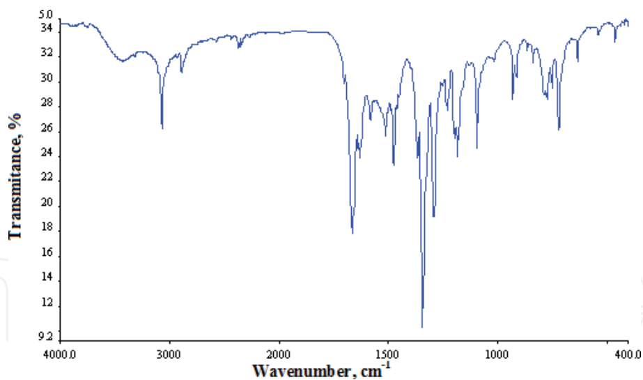
Figure 5. FT-IR spectra of ligand (2a).
