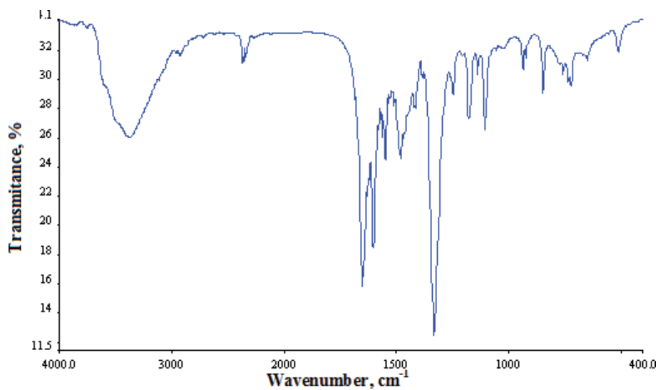
Figure 6. FT-IR spectra of Co(II) complex (3a).
