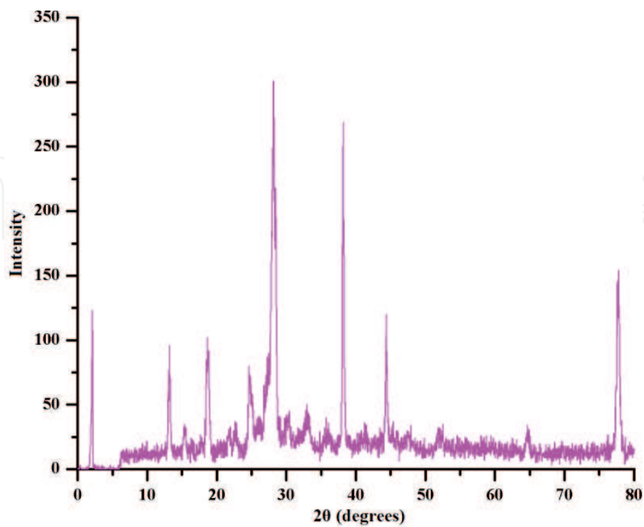
Figure 11. PXRD spectra of LH (2a).
