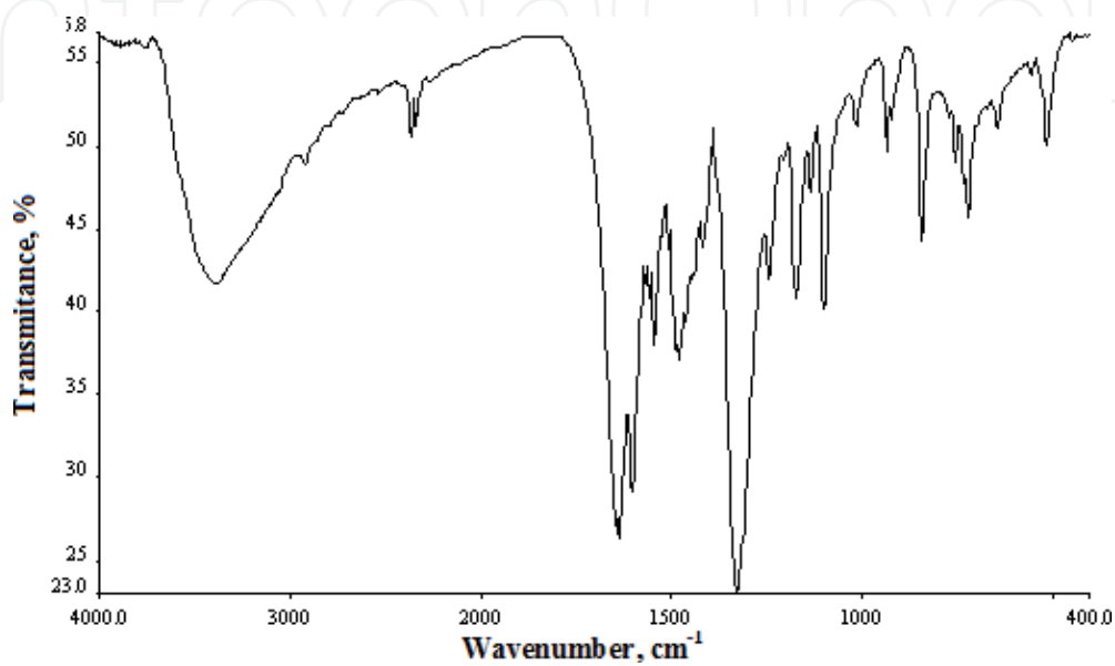
Figure 7. FT-IR spectra of Ni(II) complex (4a).
