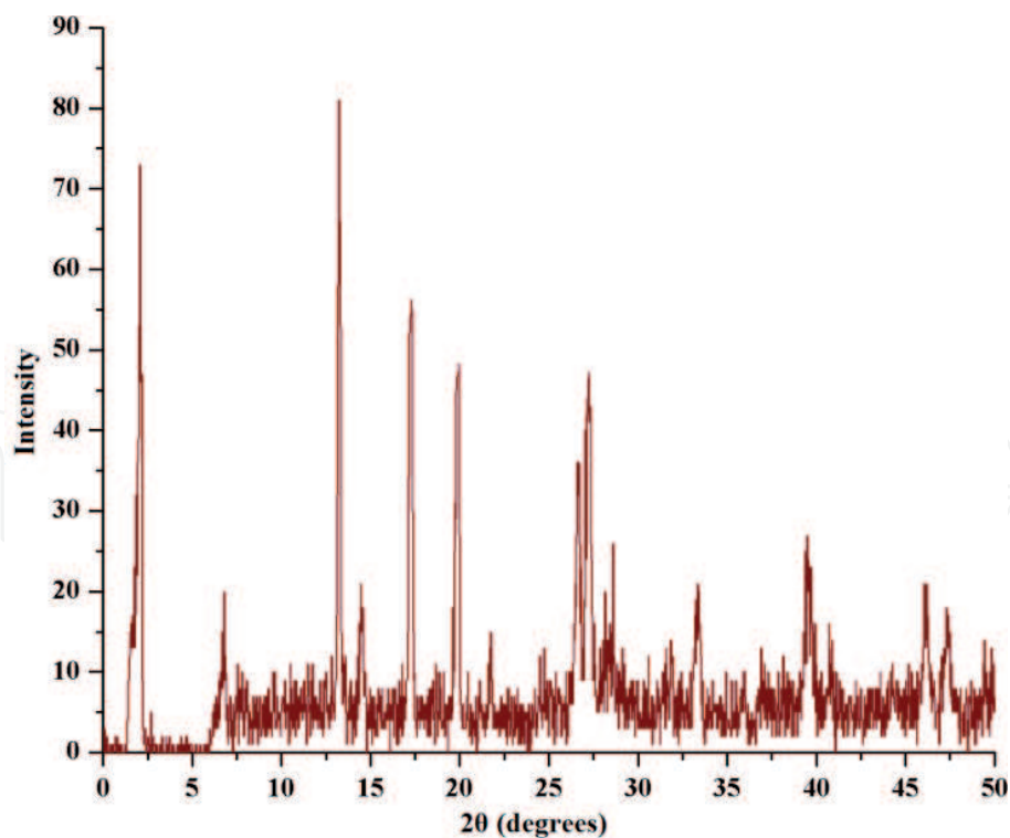
Figure 12. PXRD spectra of Co(II) complex ( 3a ).
