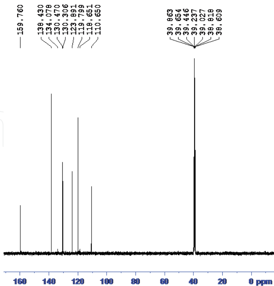
Figure 10. 13 C NMR spectra of LH (2a).
