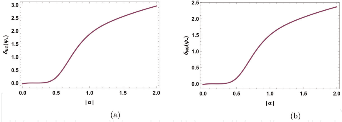
Figure 2. Non-Gaussianity versus |\alpha| . (a) for states \psi_+ and (b) for state \psi_- .
