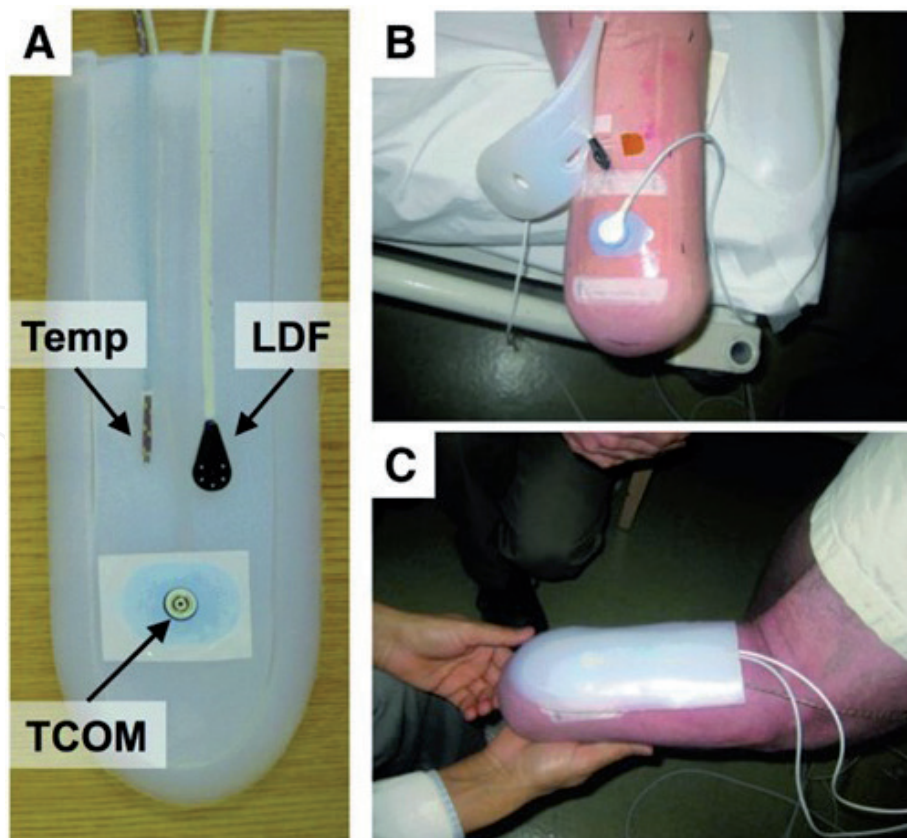
Figure 8. Silicone gel probe holder for in-liner measurement. (A) Temperature, transcutaneous oxygen measurement (TCOM) wand laser Doppler flowmetry (LDF) probes were embedded in a silicone gel insert to enable real-time measurement of limb temperature, oxygenation, and perfusion respectively. (B) Placement of probes on residual limb of transtibial participant. Oxygen permeable Tegaderm™ was used to adhere the TCOM probe to the limb. (C) The silicone gel insert enabled reproducible placement and spacing of probes and buffered against the liner from pressing probes tightly against skin (reprinted with permission from Rink et al. [33]).
