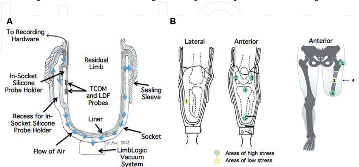
Figure 3. Elevated vacuum suspension schematic and probe measurement points. (A) Illustration of test socket with recess for in-socket silicone probe holder. (B) Residual-limb measurement sites. Green and yellow indicate measurement sites of high and low stress, respectively. LDF = laser Doppler flowmetry, TCOM = transcutaneous oxygen measurement (reprinted with permission from Rink et al. [20]).
