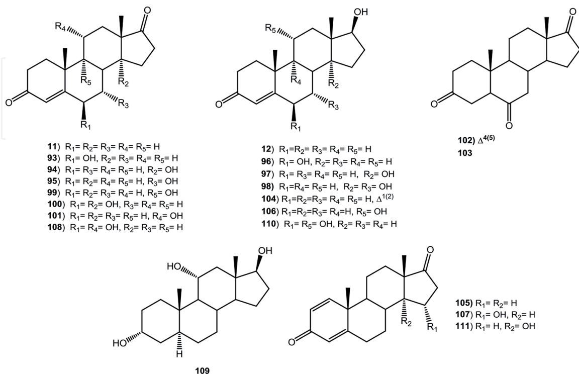
Figure 13. Biotransformation products of androst-4-en-3,17-dione (11).
