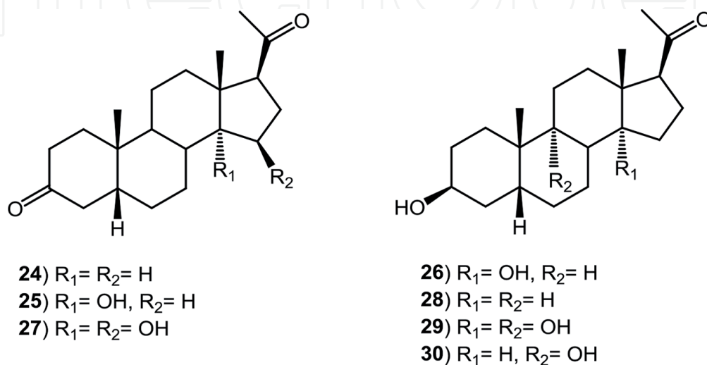
Figure 2. Biotransformation products of 5\beta -dihydroprogesterone (24).
