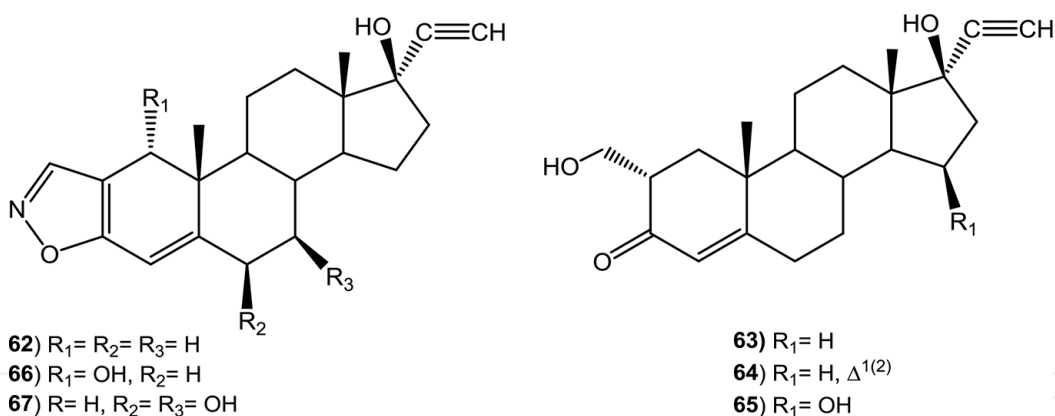
Figure 7. Biotransformation products of danazol (62)
