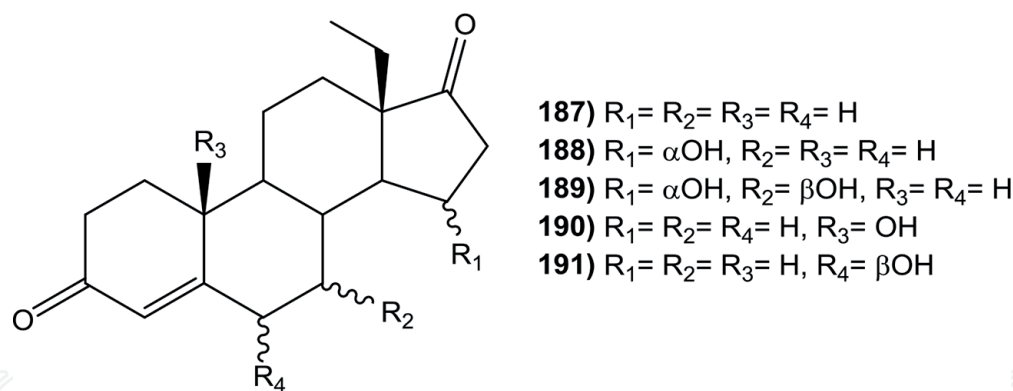
Figure 24. Biotransformation products of 13 \beta -ethyl-4-gonene-3, 17-dione ( 187 ).
