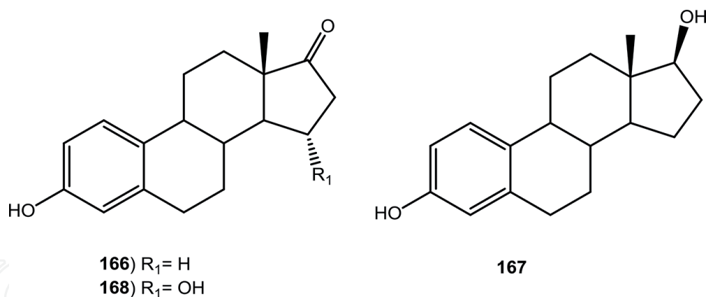
Figure 20. Biotransformation products of 3-hydroxy-1,3,5-(10)-trien-17-one ( 166 ).
