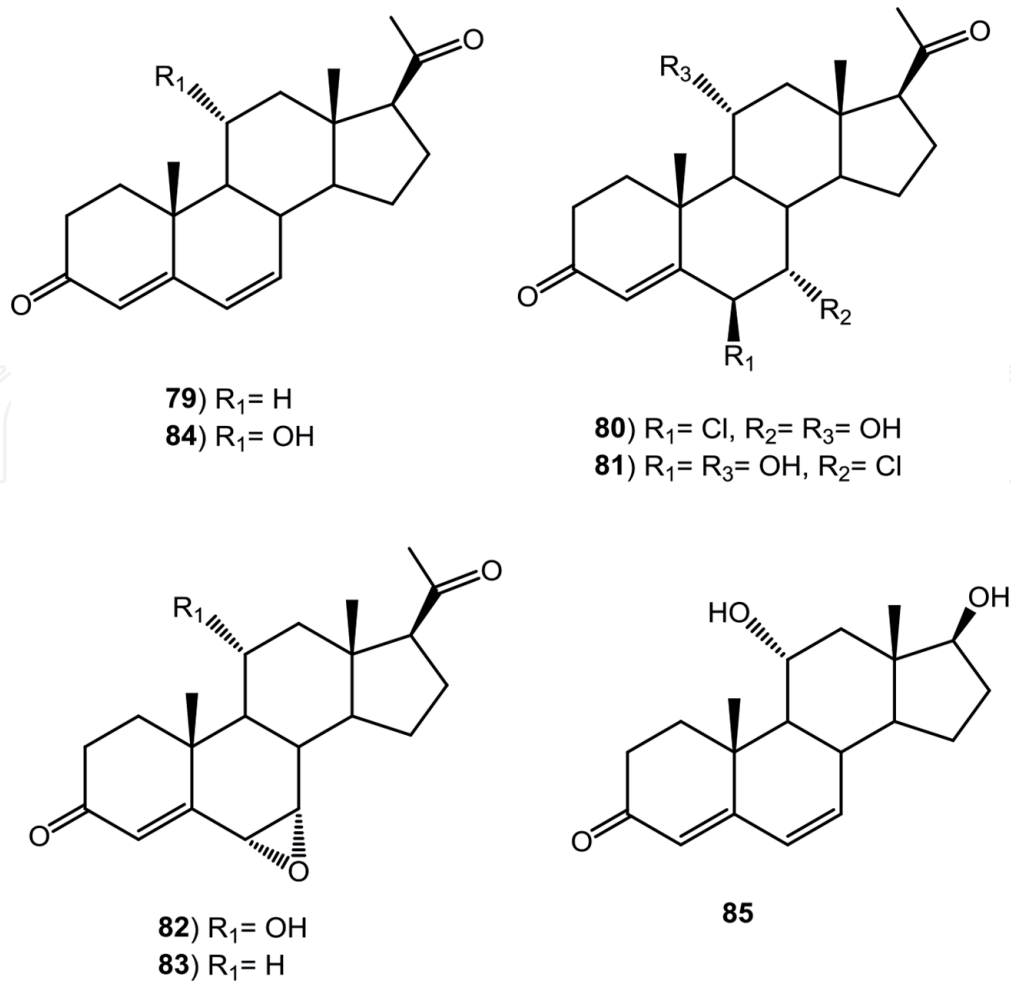
Figure 10. Biotransformation products of 6-dehydropregesterone (79).
