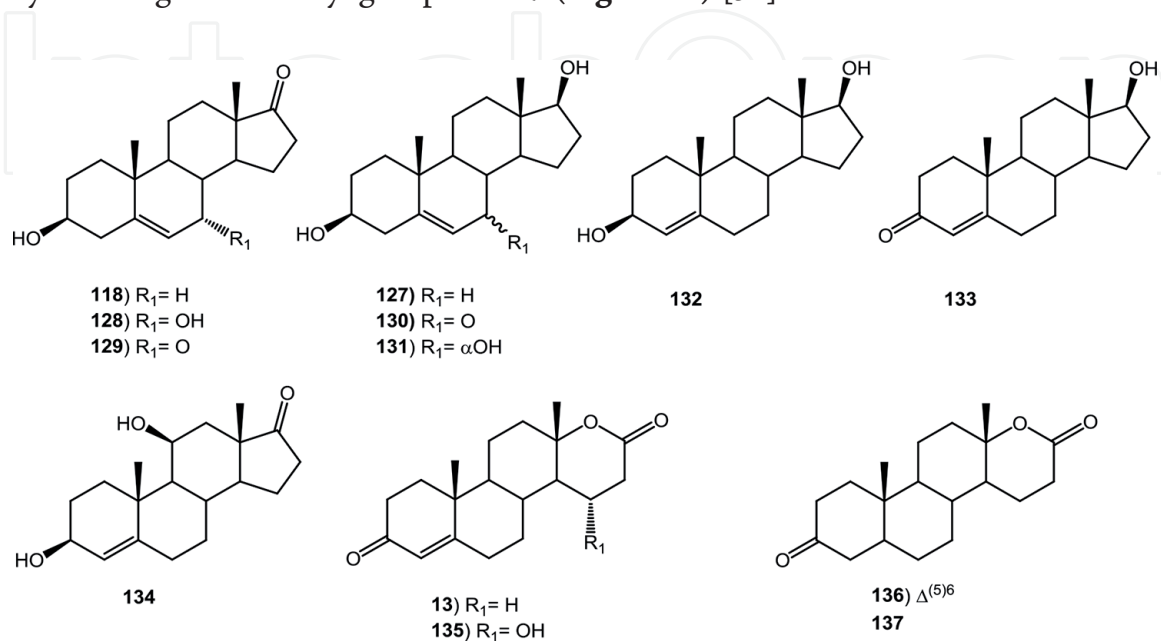
Figure 16. Biotransformation products of dehydroepiandrosterone (126).
