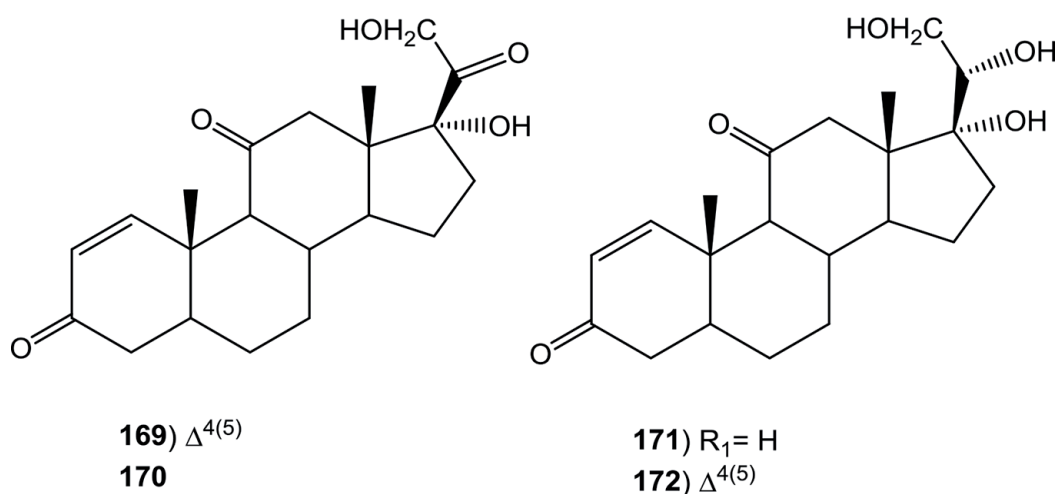
Figure 21. Biotransformation products of prednisone ( 169 ).
