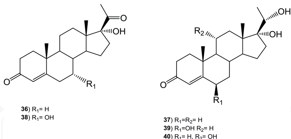
Figure 4. Biotransformation products of 17 \alpha -hydroxyprogesterone (36).
