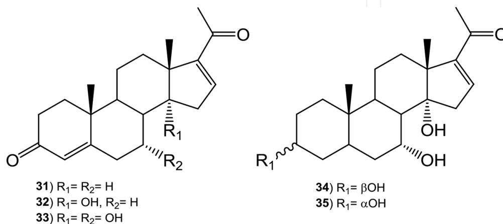
Figure 3. Biotransformation products of 16-dehydroprogesterone ( 31 ).
