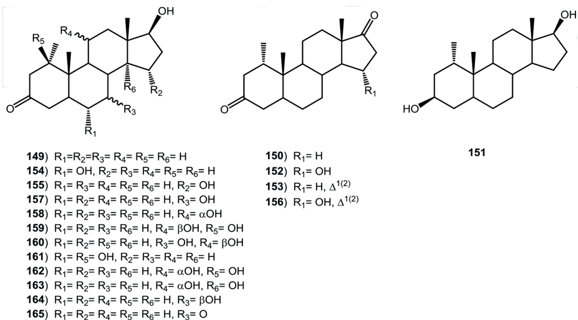
Figure 19. Biotransformation products of mesterolone (149).
