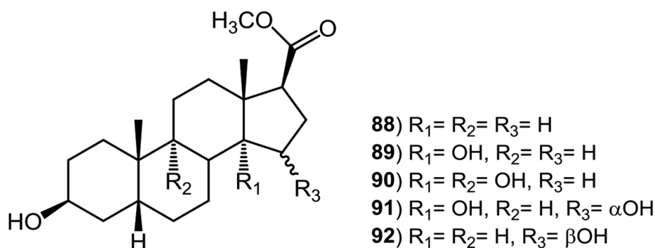
Figure 12. Biotransformation products of 3 \beta -17 \beta -carboxyethyl-5 \beta -androsteno (88).
