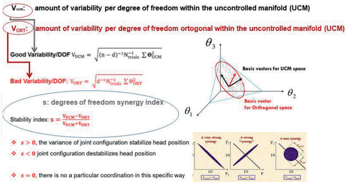
Figure 15. UCM resume.
