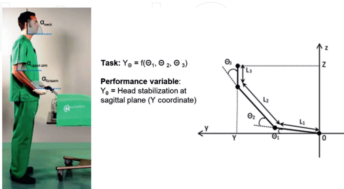
Figure 14. Mechanical UCM model.
