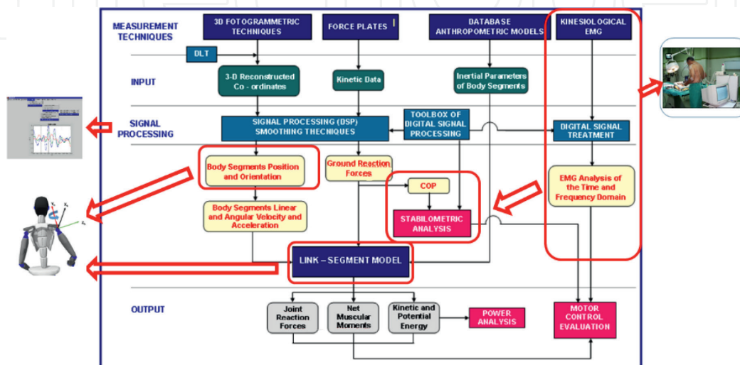
Figure 7. BiomSoft 2.0 flow chart.
