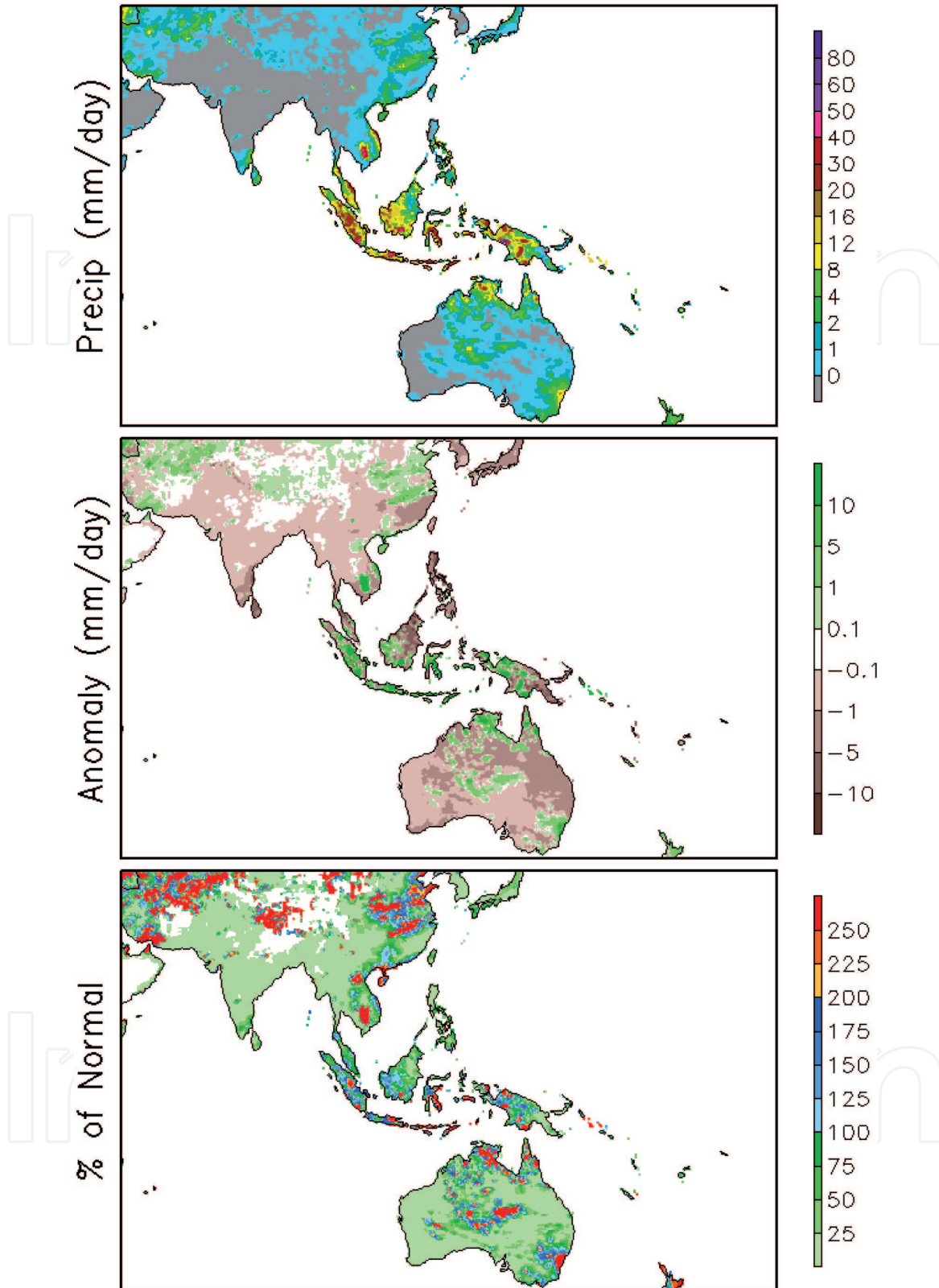
Figure 3. CPC/NOAA CMORPH weekly summary: mean precipitation, mm/day (top panel); precipitation anomaly, mm/day (middle panel); and precipitation percentage of normal, % (bottom panel) for a week from November 26, 2018 to December 2, 2018.
