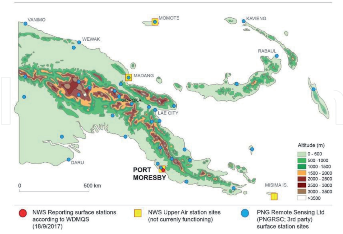
Figure 8. Schematic map of Papua New Guinea depicting topographic extremes and the observations received from the NWS surface network on the morning of September 18, 2017, the NWS historically active upper air station sites (not currently functioning) and the location of 37 PNG Remote Sensing Centre Ltd. automated weather station sites (third party privately owned).
