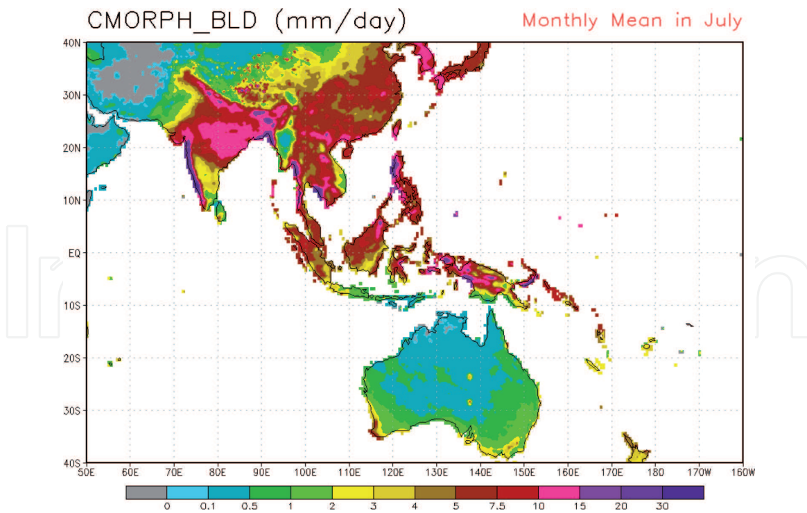
Figure 2. CPC/NOAA CMORPH monthly mean precipitation (climatology) for July (1998–2017 base period).
