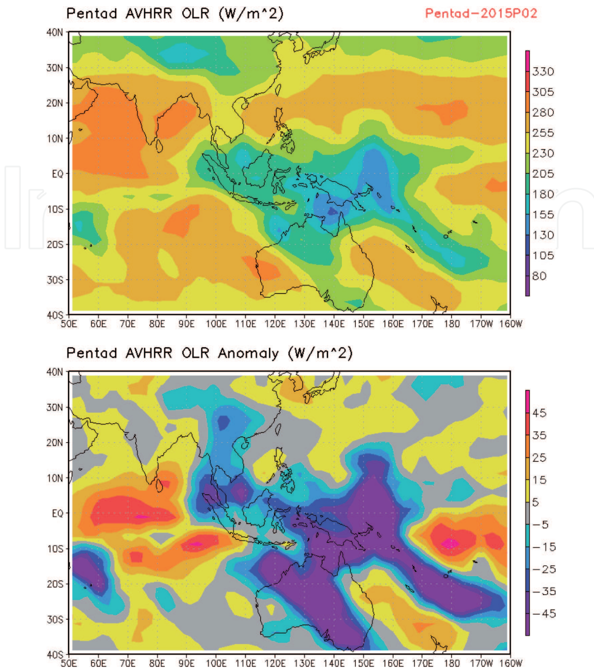
Figure 6. AVHRR OLR for January 6–10, 2015, i.e. pentad 2 (top panel) and pentad OLR anomaly (bottom panel), W/m 2 .
