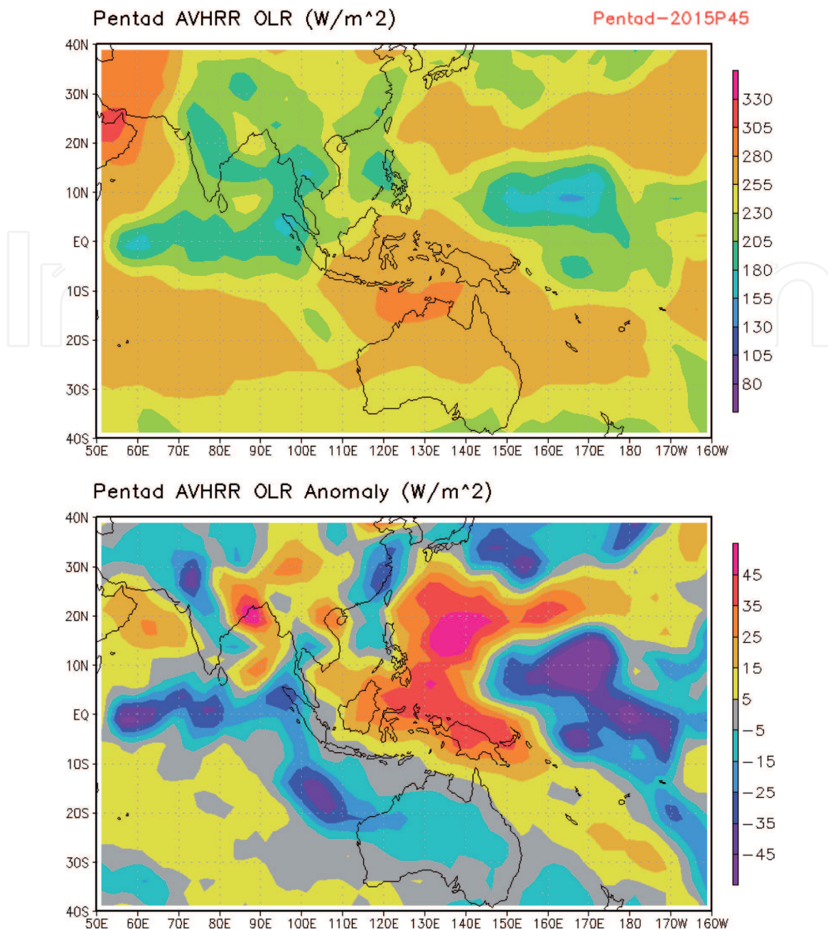
Figure 7. AVHRR OLR for August 15–19, 2015, i.e. pentad 45 (top panel) and pentad OLR anomaly (bottom panel), W/m 2 .
