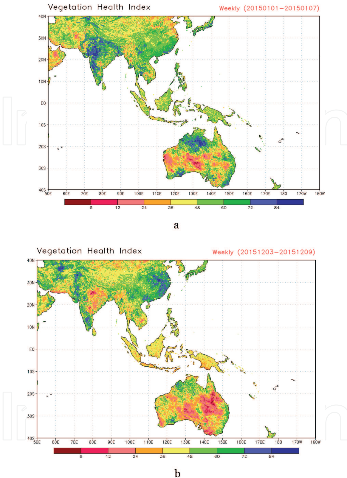
Figure 5. CPC/NOAA CMORPH VHI for January 1–7, 2015 (top panel) and December 3–9, 2015 (bottom panel).
