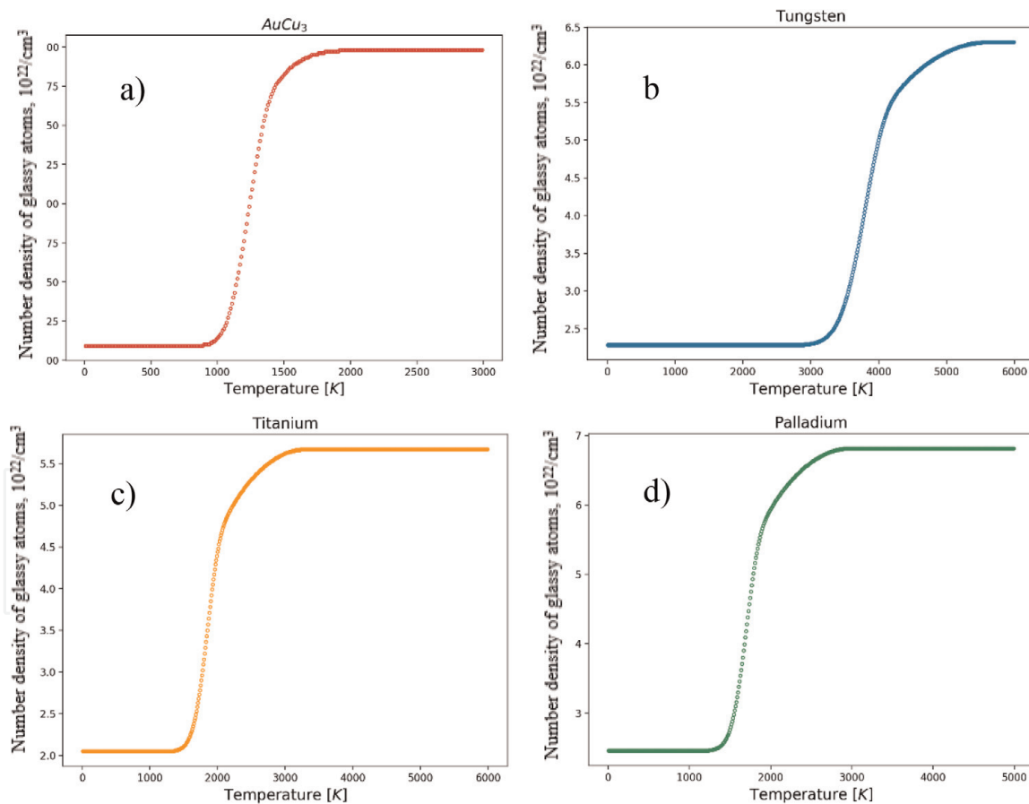
Figure 1. Calculated number of glassy state atoms per cc as a function of temperature for: (a) binary alloy—AuCu 3 (1240.5 K); (b) BCC—tungsten (3695 K); (c) HCP—titanium (1948 K); and (d) FCC—palladium (1828 K). The melting points of the metals are listed in the parentheses. Operationally, we take the melting point to be at midpoint between the minimum and the maximum of the number density of glassy atoms, and this is in good agreement with the known data. By taking the midpoint between the maximum and the minimum number density. At room temperature when the population of nanocrystallites is largest, in each plot the number density of glassy state atoms starts off at the particular value, corresponding to its own randomly close packed state. In the case of AuCu 3 the number density of glassy state atoms at room temperature is 4.1 \times 10^{22} atoms per \text{cm}^3 . The rest of the atoms are tied up in the form of nanocrystallites with the degree of crystallinity at 0.314; the number of glassy state atoms increases to 5.98 \times 10^{22} atoms per \text{cm}^3 when the specimen is fully molten [4].
