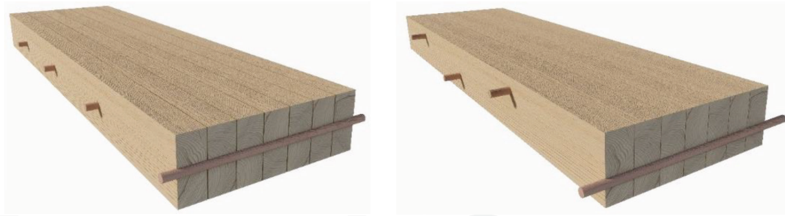
Figure 13. DLT with linear (left) and staggered (right) fastening patterns.
