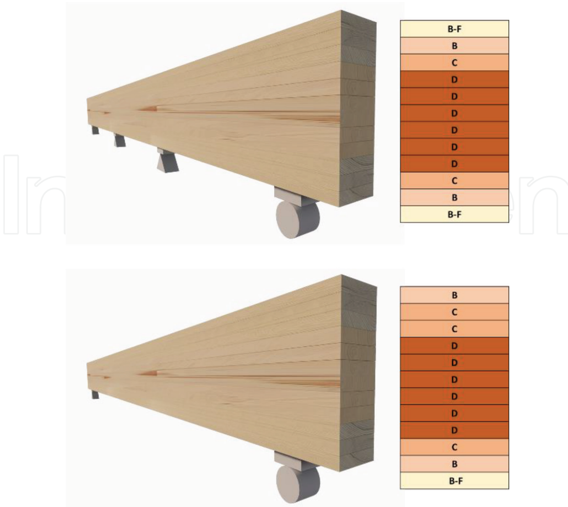
Figure 5. GLT members with laminations suiting resistance of bending forces: Upper—Member with a balanced layup intended to maximize material use when the member is loaded in tension on both top and bottom faces (EX grade under Canadian system), and Lower—Member with an unbalanced layup intended to maximize material use when the member is loaded in tension on the bottom face (E grade under Canadian system).
