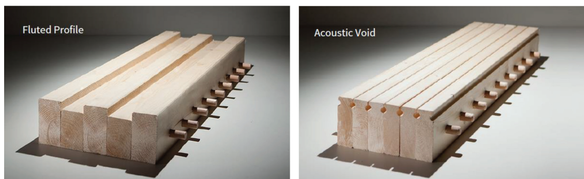
Figure 14. Two sample profiles of DLT (Source: Pictures obtained from StructureCraft [18]).
