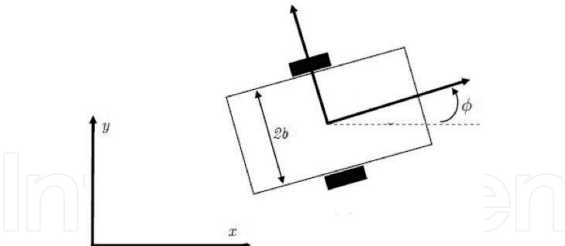
Figure 1. Wheeled mobile robot.
