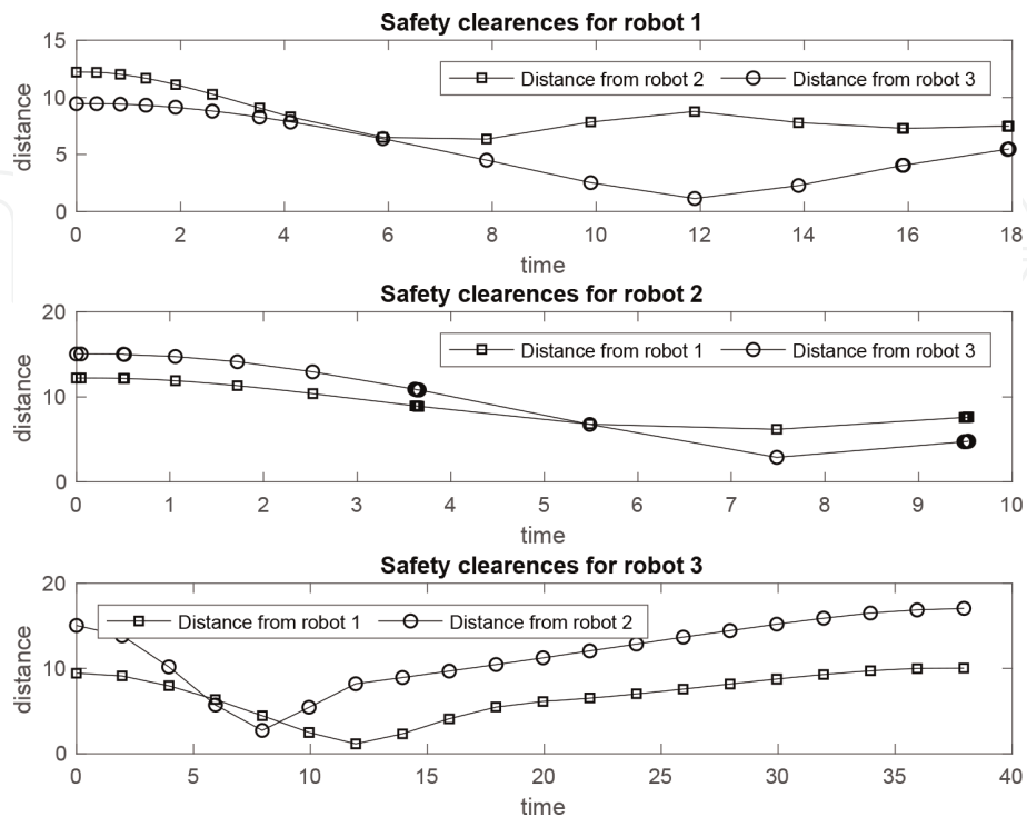
Figure 4. Collision avoidance (Example 1).
