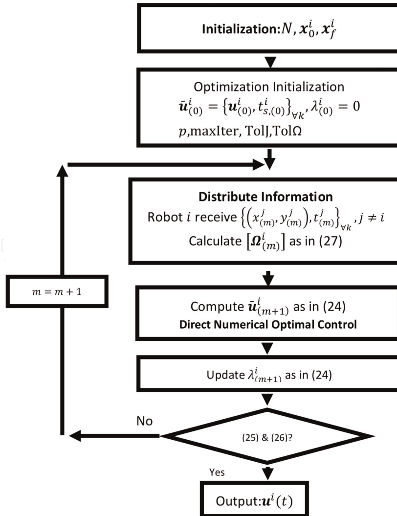
Figure 2. Distributed algorithm flowchart to optimize multi-robot motion.
