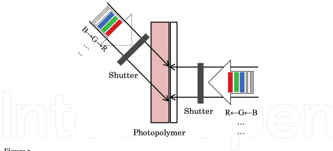
Figure 5. Schematic of a multicolor reflection HVG recording.
