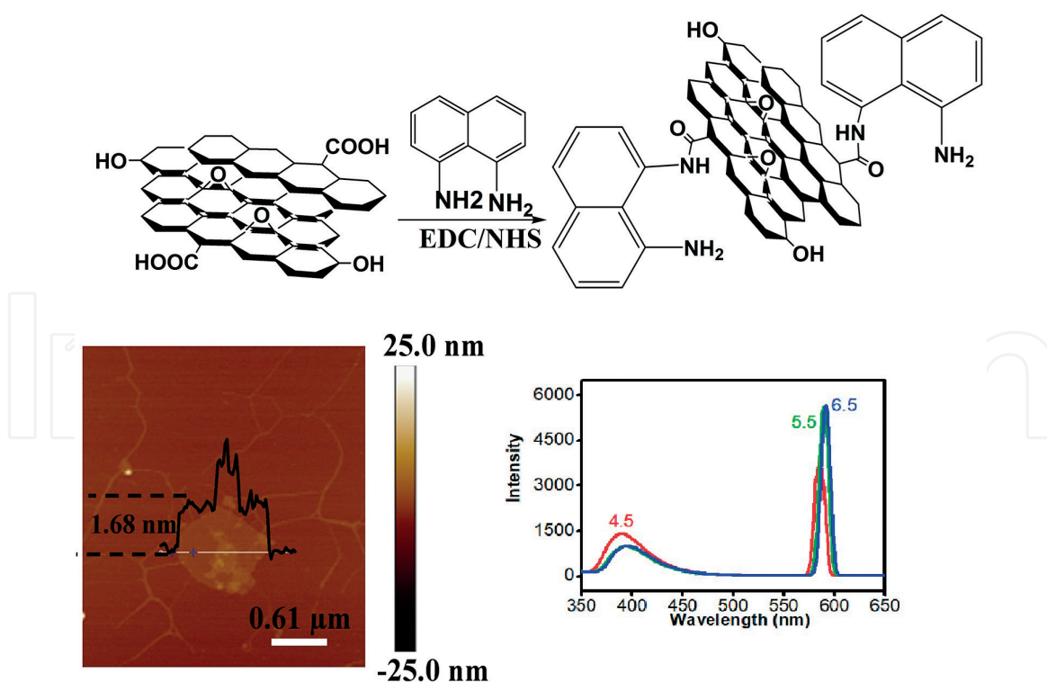
Figure 4. Synthetic pathway and AFM images of GAP and its fluorescence response to fivefold Ag + in aqueous solutions with various pHs.
