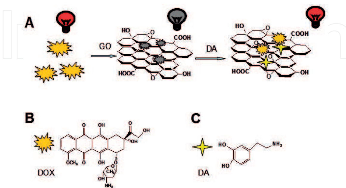
Figure 3. A schematic illustration of the fluorescence response of a DOX-GO complex to dopamine (a); Molecular structures of DOX (b) and dopamine (c).
