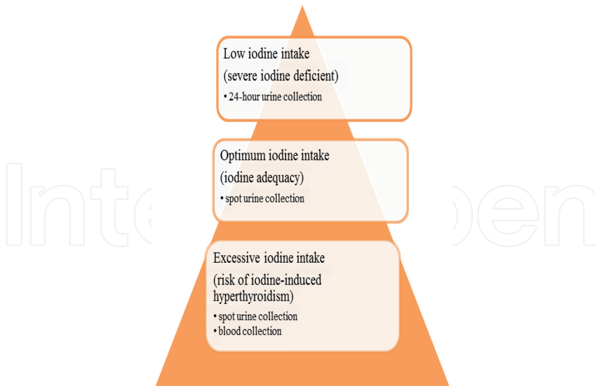
Figure 1. Degrees of iodine intake (iodine nutrition status) and their suitable types of human sample collection to determine the median urinary iodine concentration (mUIC).
