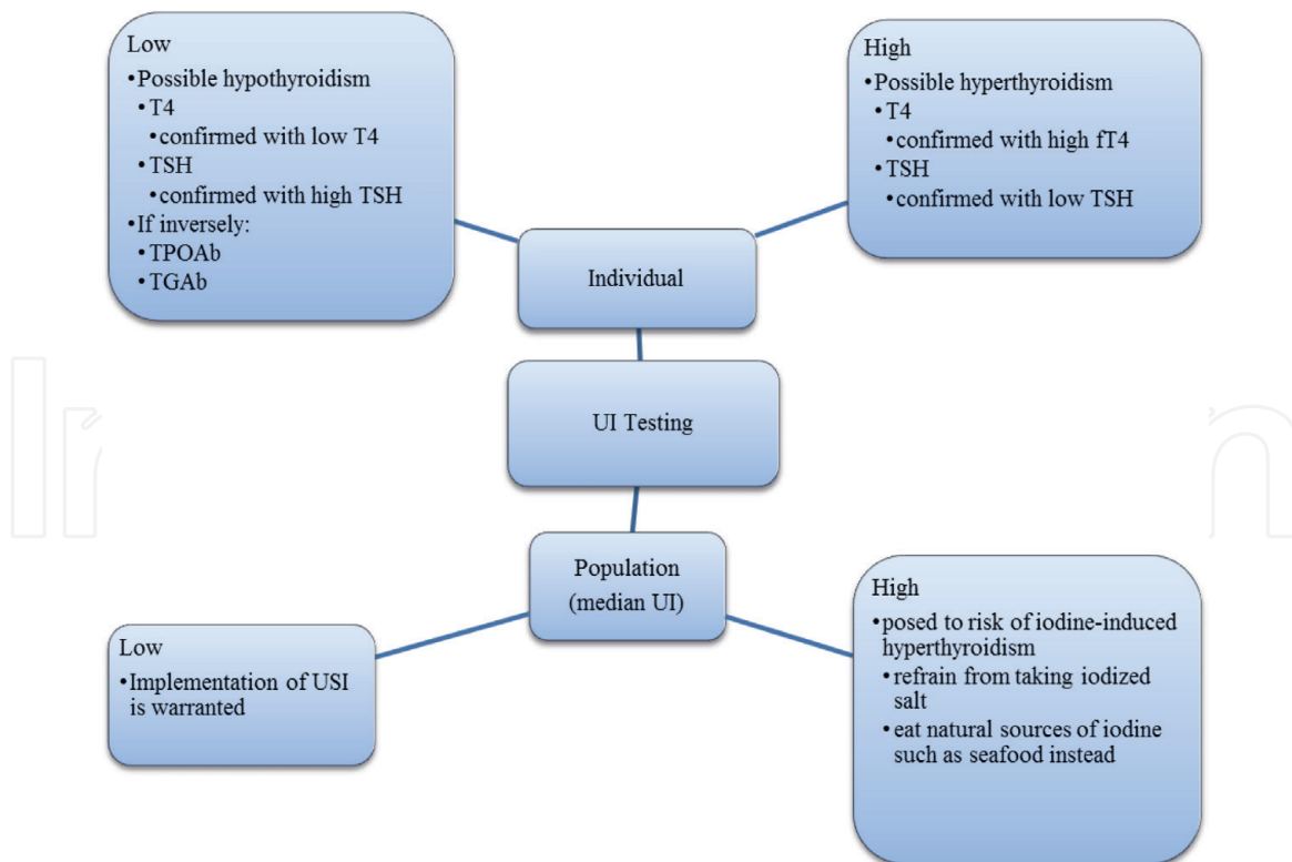
Figure 4. Subsequent biomarker testing and further action for individual and population urinary iodine estimation.
