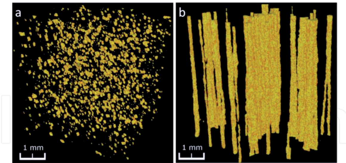
Figure 10. Exemplary X \mu CT images of the isotropic (a) and anisotropic (b) MRE samples with \sim 5 wt% magnetic particles. [67].
