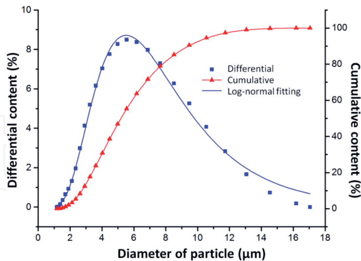
Figure 3. The size distribution of carbonyl iron powder (Type CIP-CN) [46].
