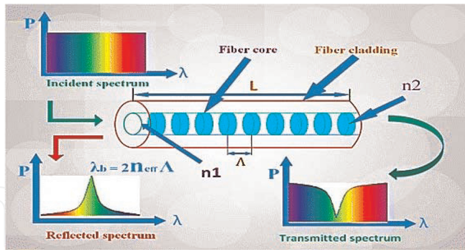
Figure 1. Basic structure of fiber Bragg grating.
