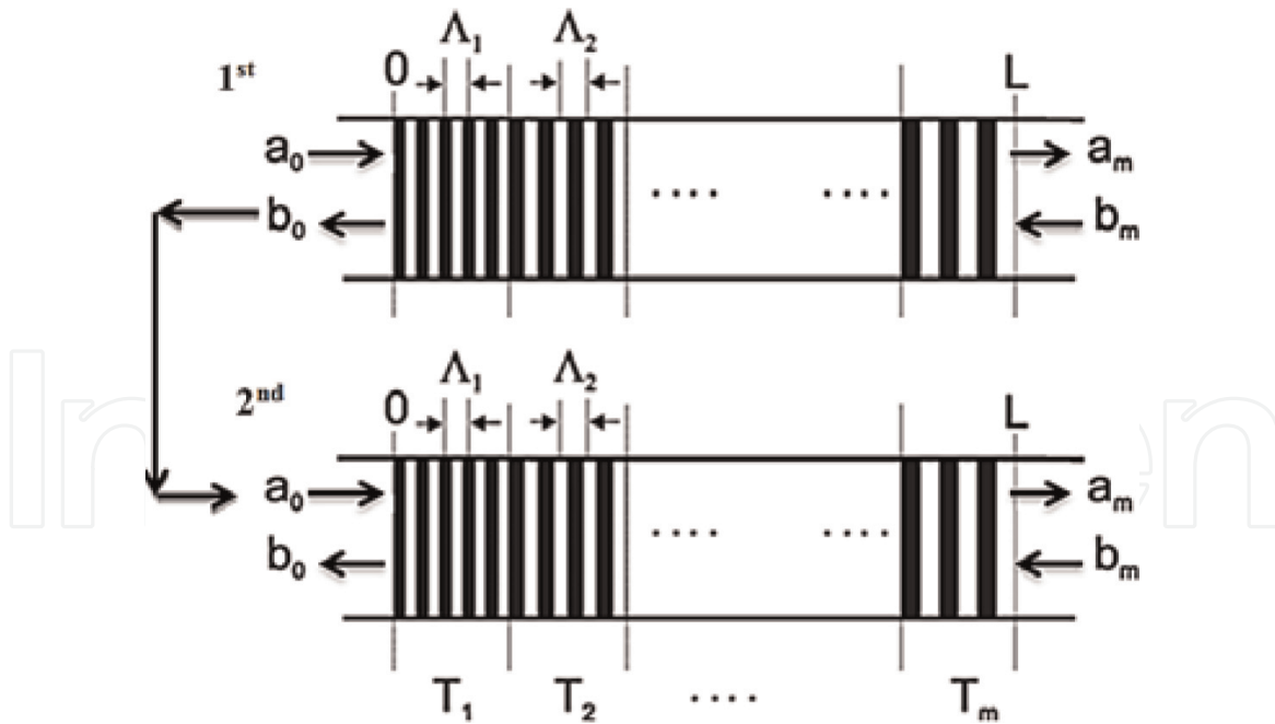
Figure 3. Connection between two cascaded FBG.
