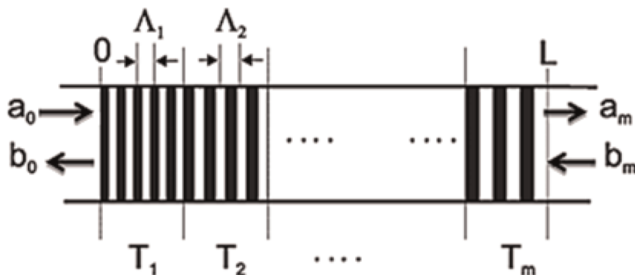
Figure 2. Fiber Bragg grating sections.
