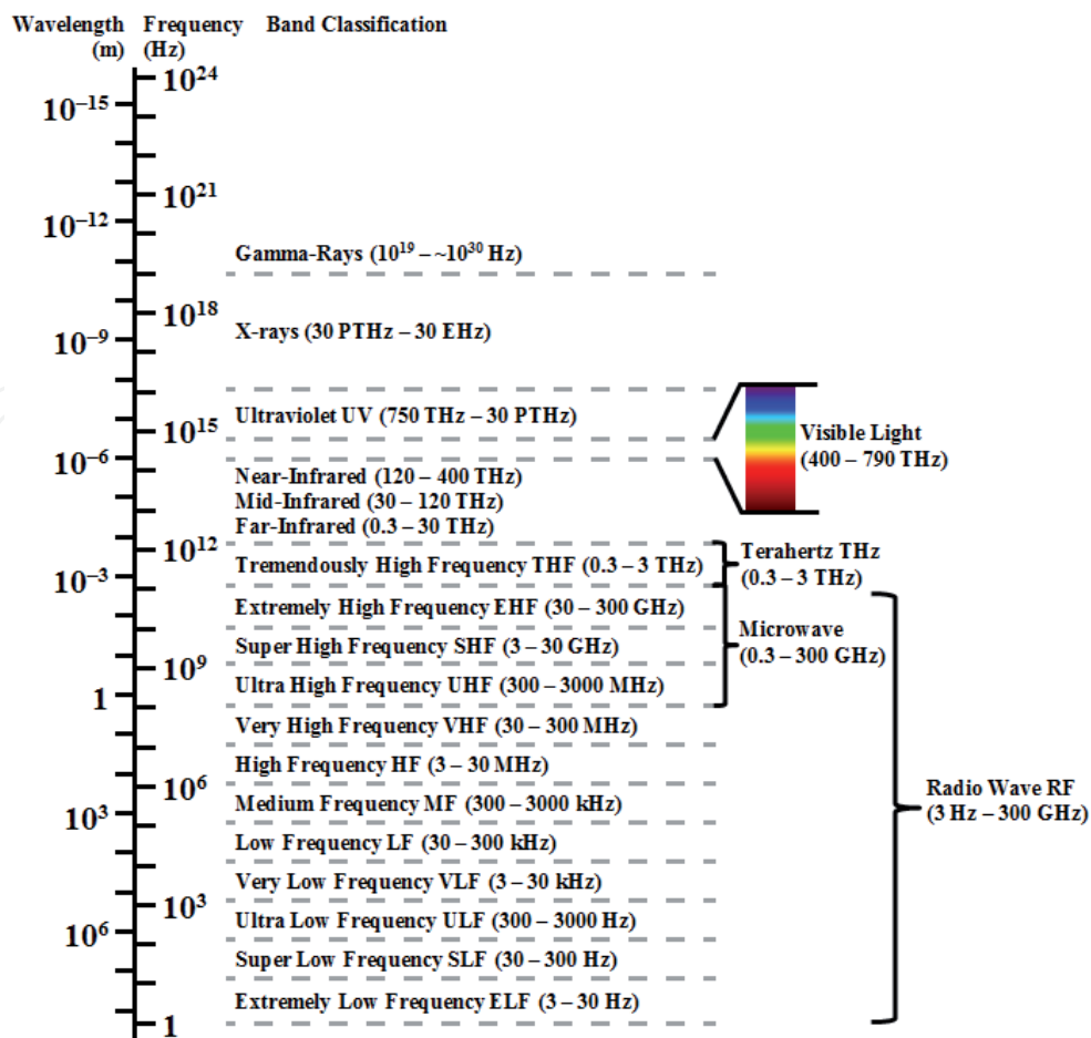
Figure 2. The electromagnetic spectrum.
