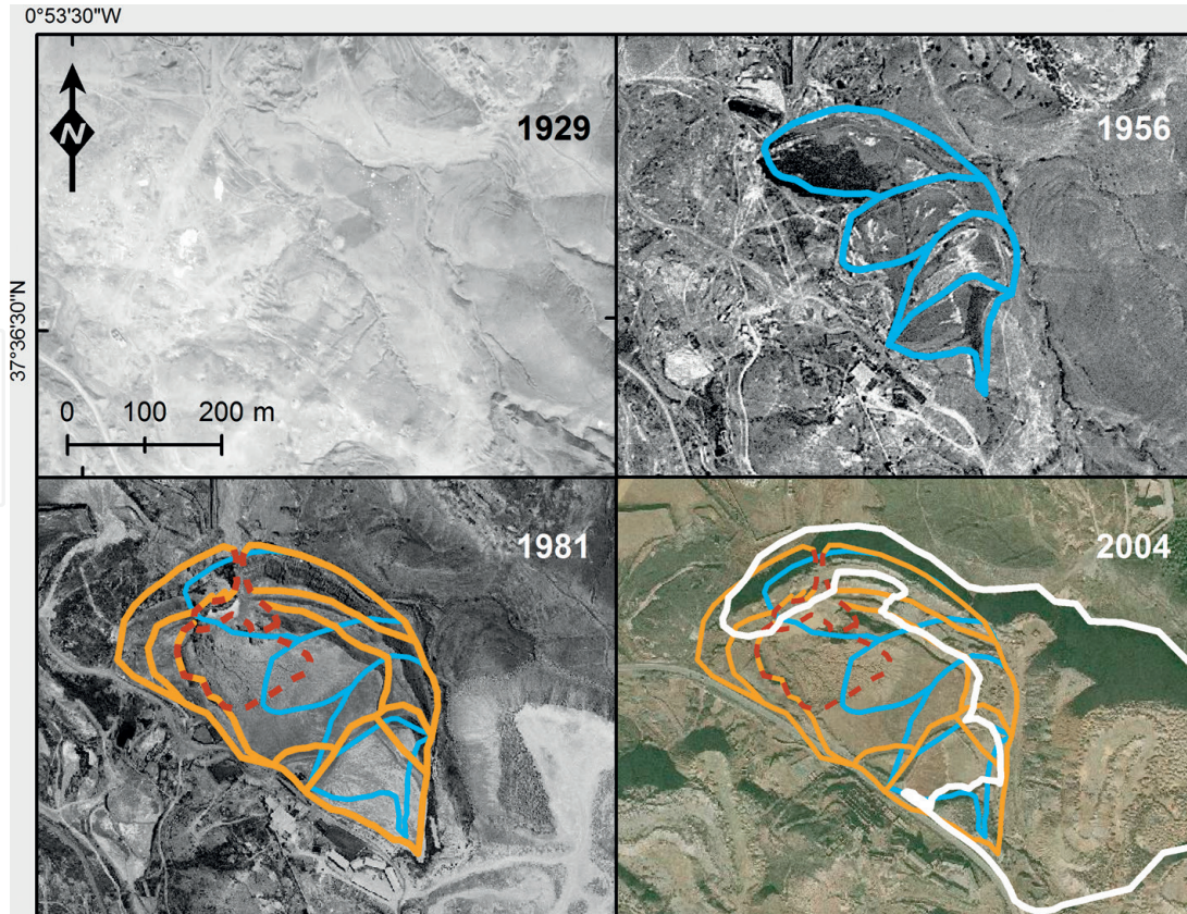
Figure 6. Landscape evolution in the surroundings of the Brunita mine pond from aerial photographs taken in: 1929 (Ruiz de Alda photogrammetric flight); 1956 (Geographic Service of the Spanish Army); and 1981 and 2004 (Spanish National Geographic Institute). Blue lines, mine ponds in 1956; orange lines, mine ponds in 1981; brown dashed lines, badlands and landslide scar in 1981; and white line, spoil tips in 2004.
