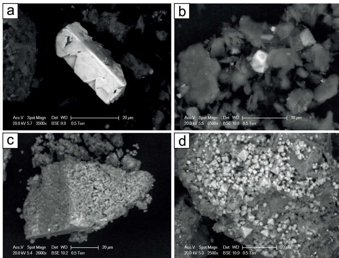
Figure 2. Backscattered electron (BSE) images: (a) galena crystal from Monte Romero; (b) pyrite crystal from San Quintín; (c) altered faces of a pyrite crystal from San Cristóbal; (d) subidiomorphic magnetite from Las Moreras.
