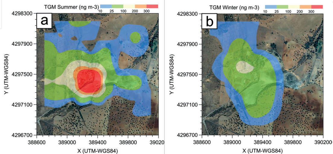
Figure 3. Total gaseous mercury (TGM) seasonal distribution in the San Quintín area: (a) summer and (b) winter values. Modified from Martín-Crespo et al. [6].
