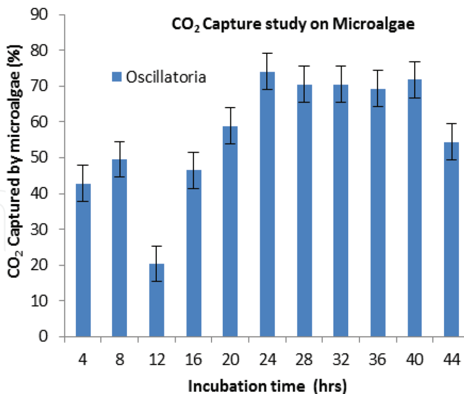
Figure 6. CO 2 capture by Oscillatoria .
