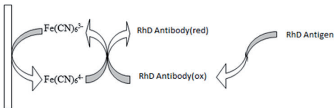
Figure 1. The principle of the biosensor [26].
