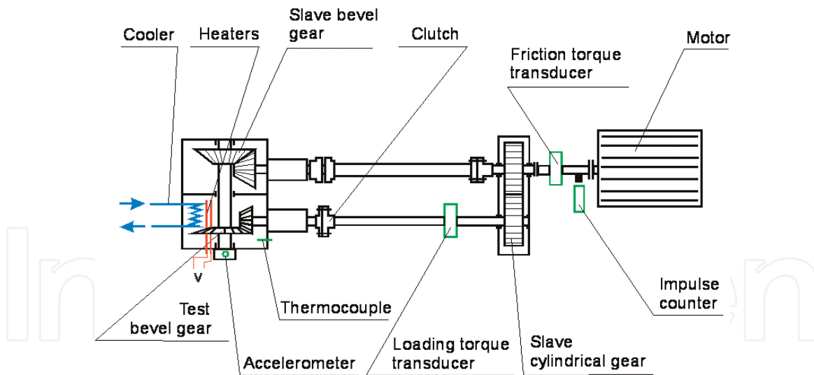
Figure 7. Kinematic scheme of the T-30 back-to-back bevel gear test rig.
