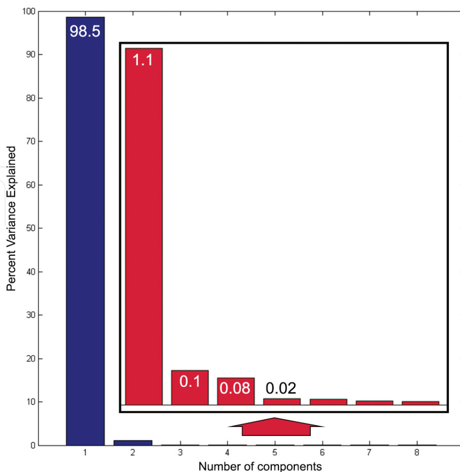
Figure 3. Result of PCA analysis showing the contribution of the first principal components highlighted in blue color.
