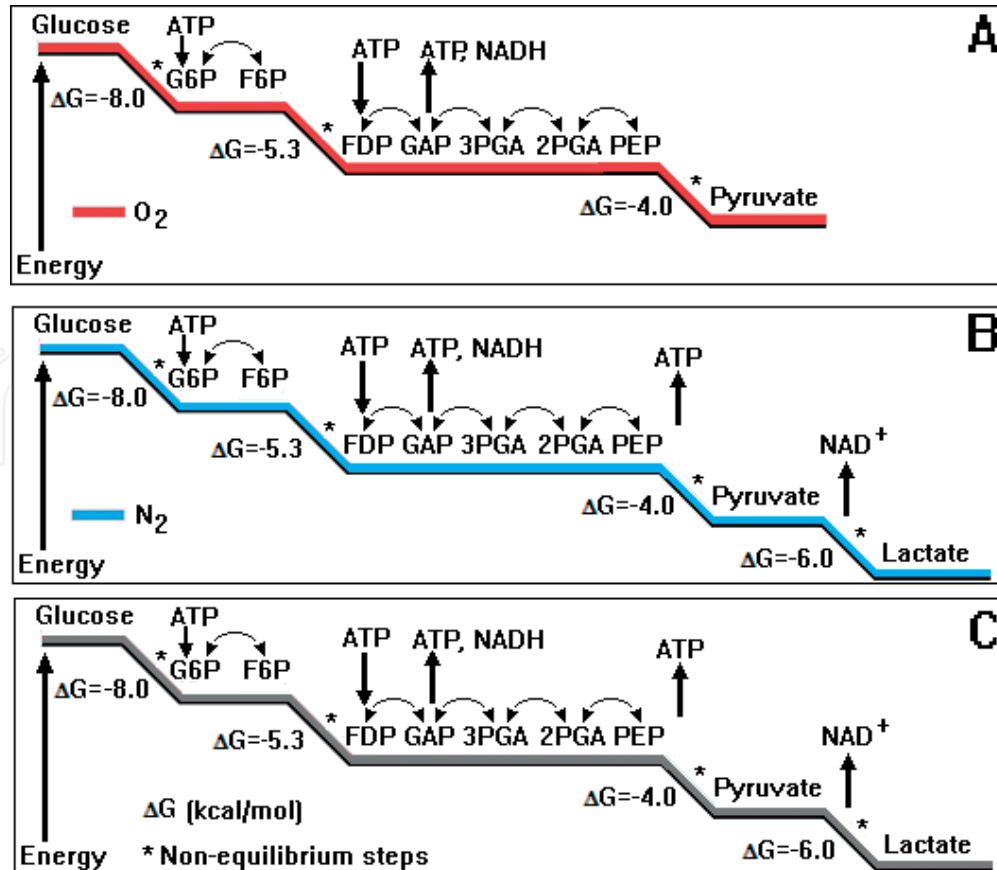
Figure 2. A schematic illustration of the potential free-energy change profile of aerobic (A) and anaerobic glycolysis (B). The potential free-energy change of the reaction pyruvate \rightarrow lactate dictates that it should proceed regardless of the oxygenation conditions (C).
