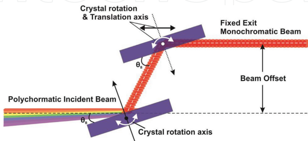
Figure 6. Geometry of fixed-exit double-crystal monochromator (DCM) system.
