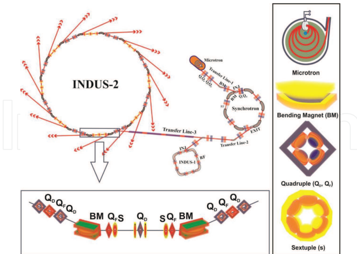
Figure 1. Detailed outer structure of RRCAT—Indian third-generation synchrotron light source. Electrons are generated via microtron and transferred to the synchrotron for making an accelerated e^- -beam. The energetic e^- -beam has been introduced to the Indus-1 and Indus-2 via transfer lines. The beam optics have been maintained by the periodic repetition of several magnetic components (quadruple focused ( Q_F ), quadruple defocused ( Q_D ), sextuple ( S ), and bending magnets ( BM )) to force e^- beam to follow a circular path.
