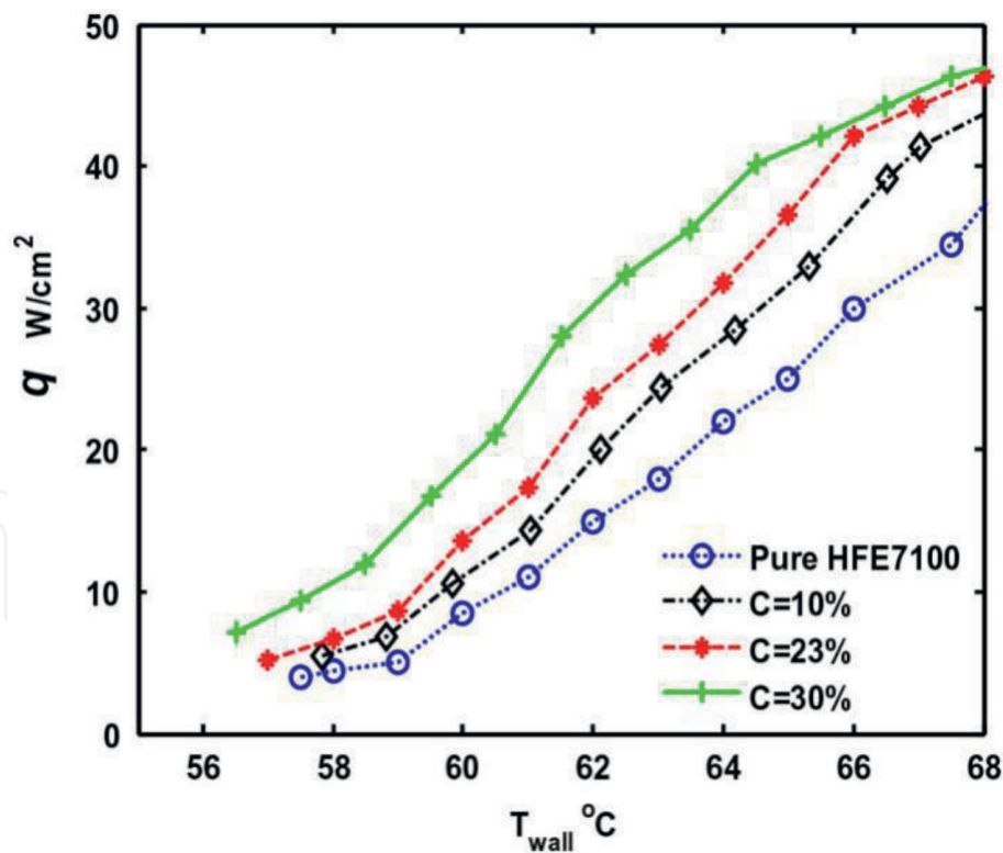
Figure 10. HFE7100 jet impingement (56–68°C) heat flux at the flow rate of 7.15 cc/s; (note: the inlet T_{in} was controlled at 56°C, nozzle: TGo.76, H = 20 mm). Slurry with 30% particle mass fraction improved average heat transfer coefficient by 70% when compared to pure HFE7100 for jet impingement at the temperature range from 62 to 66°C.
