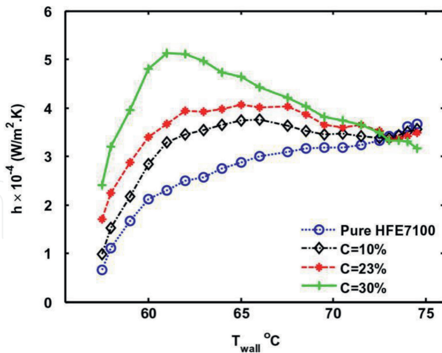
Figure 12. Heat transfer coefficients of slurry with 30% particle mass fraction vs. heater surface temperature of full range (56–75°C) at the flow rate of 7.15 cc/s (note: the inlet T_{in} was controlled at 56°C, nozzle: TGo.76, H = 20 mm).
