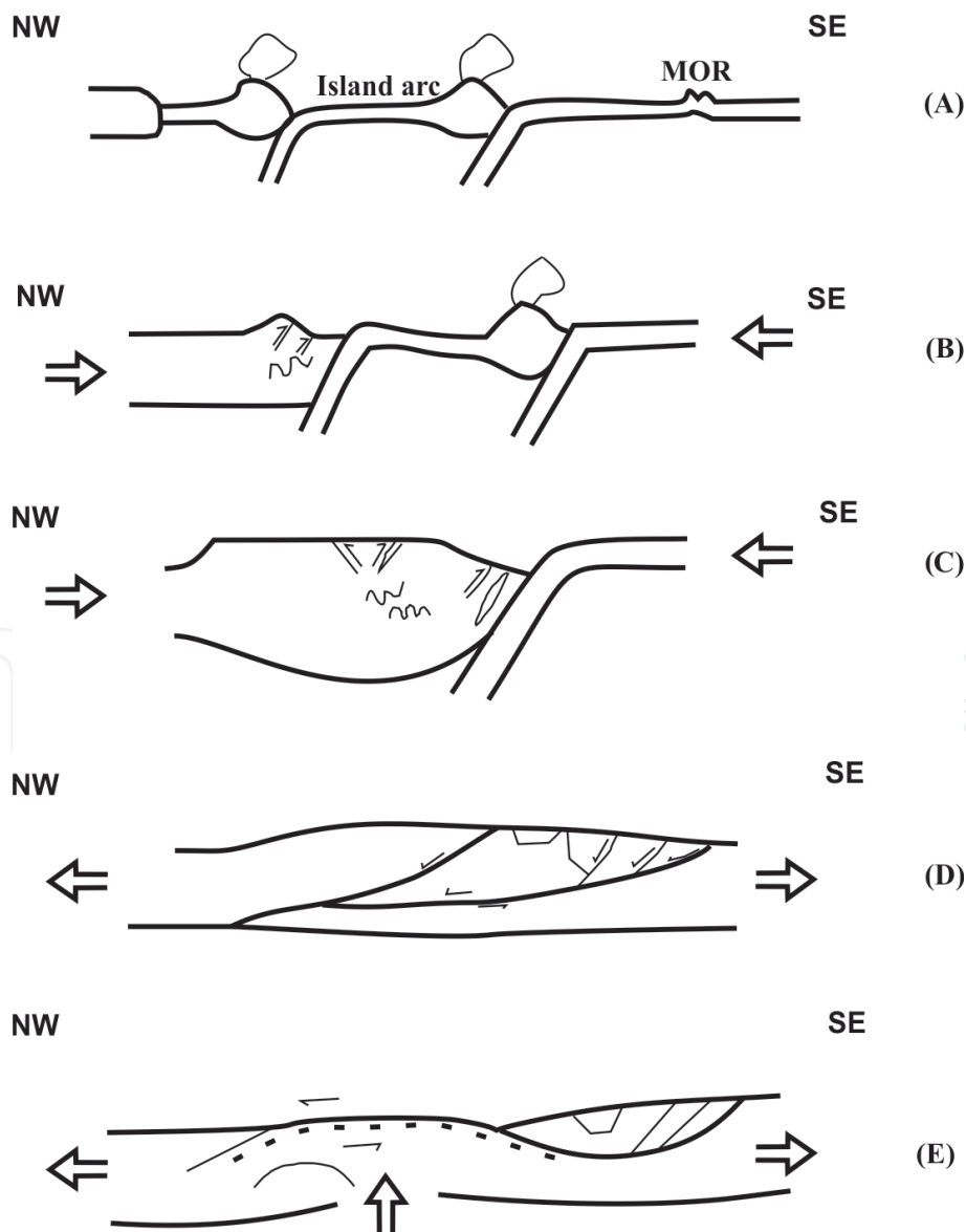
Figure 8. A cartoon displaying the different stages of the evolution of the Arabian-Nubian Shield after [88].
