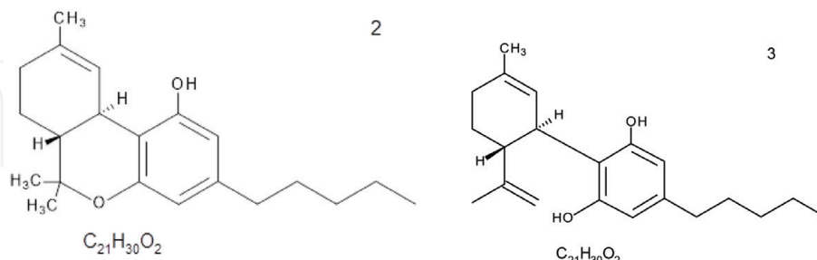
Figure 4. (1) Marijuana ( Cannabis sativa ), (2) diagram of THC, tetrahydrocannabinol, (3) diagram of CBD, cannabidiol.
