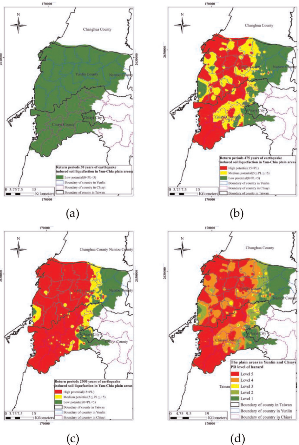
Figure 5. Three different return periods of earthquake forces and Hazard distribution condition. (a) Soil liquefaction for earthquakes with a 30-year return period, (b) Soil liquefaction for earthquakes with a 475-year return period, (c) Soil liquefaction for earthquakes with a 2500-year return period, and (d) Hazard level induced by soil liquefaction.
