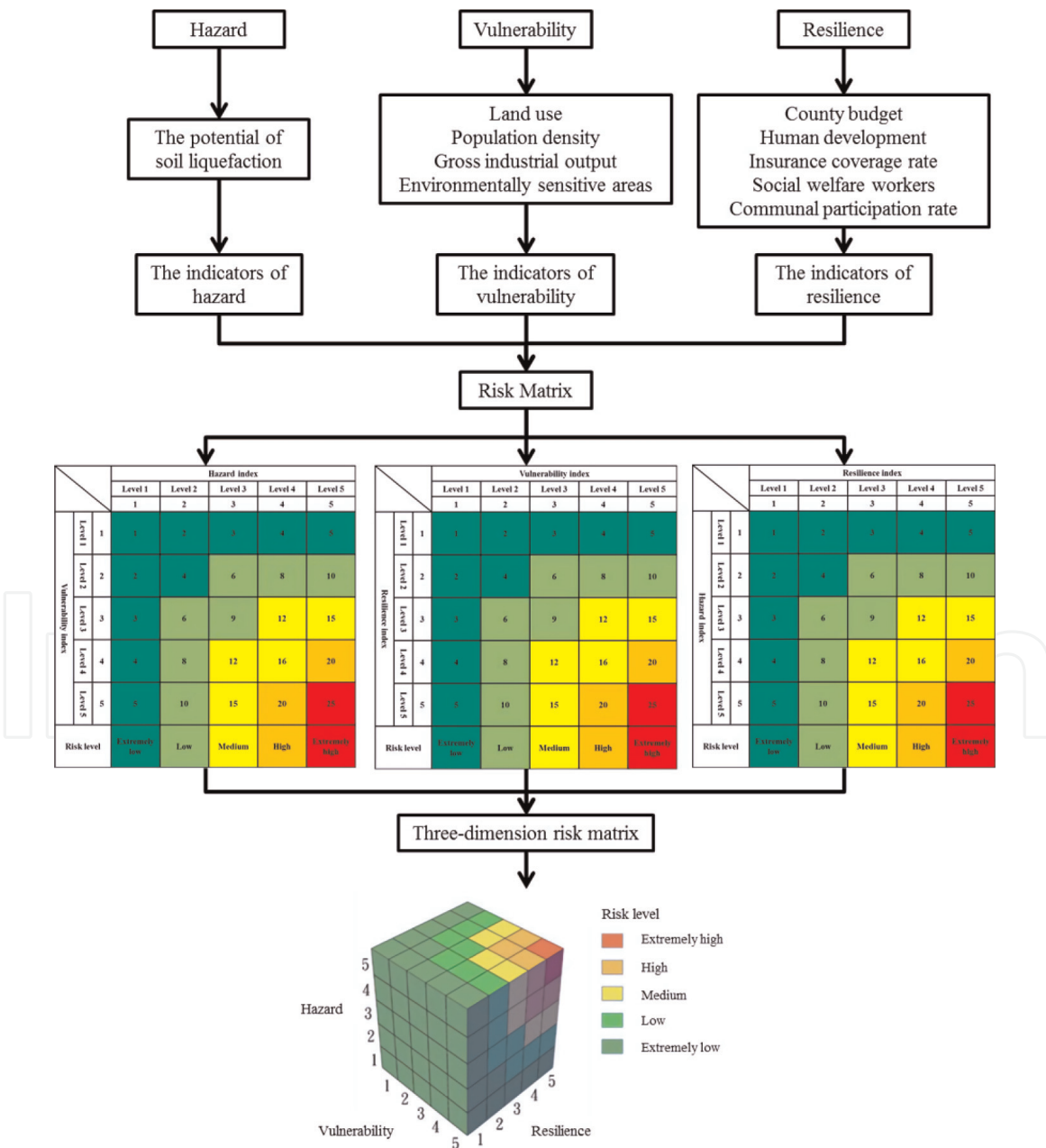
Figure 8. Procedure of the risk level analysis.
