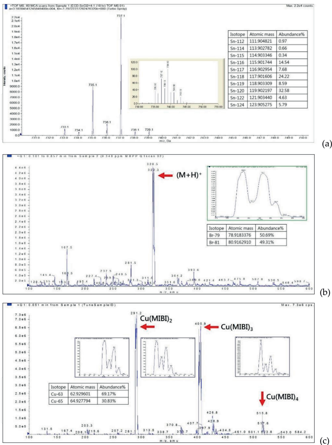
Figure 9. Stable isotope distribution patterns and simulation of mass spectra of (a) Sn(ECD) 2 (DP#4), (b) (R)-N-methyl-3-(2-bromophenoxy)-3-phenylpropanamine (MBPP), and (c) methoxyisobutylisonitrile (sestamibi).
