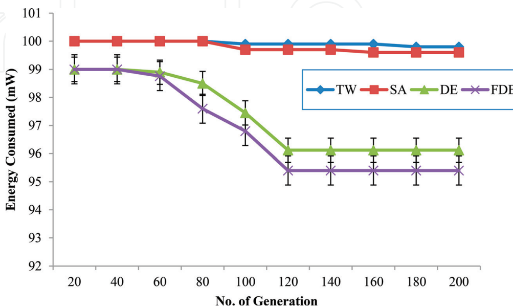
Figure 6. Energy consumption of mesh nodes.
