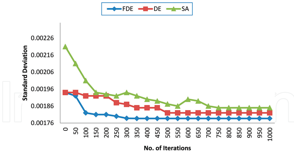
Figure 8. Convergence rate.
