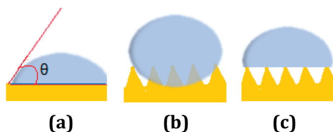
Figure 1. Comparison between wetting regimes: (a) Young, (b) Wenzel, and (c) Cassie.
