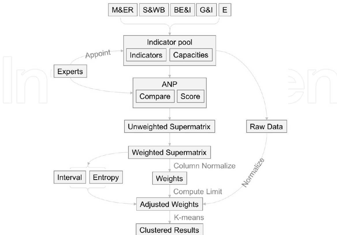
Figure 1. Decision-making flow.
