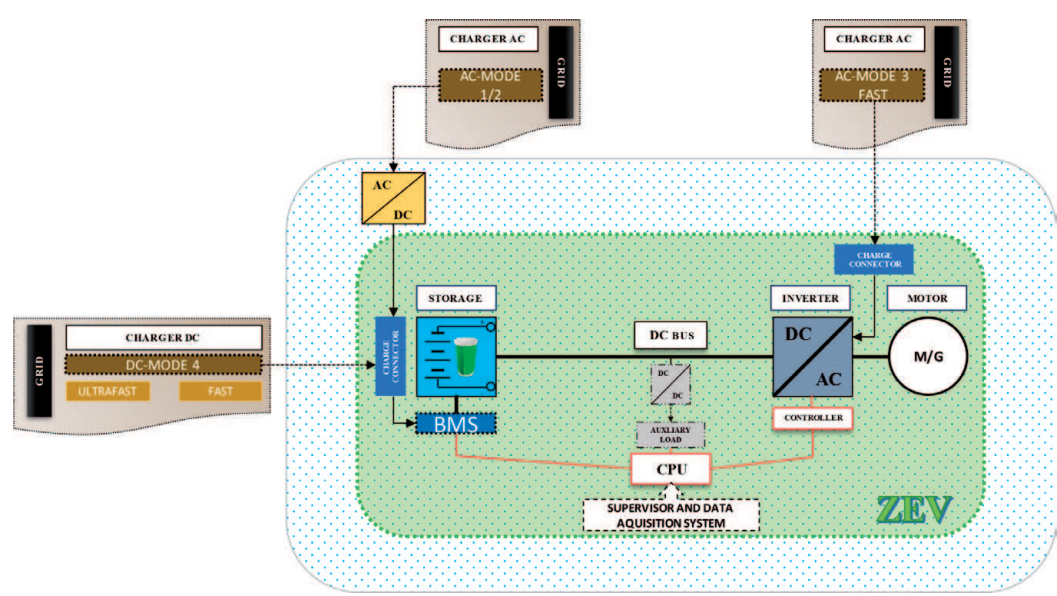
Figure 11. Electric drive architecture for ZEV: single-stage converter/single motor.
