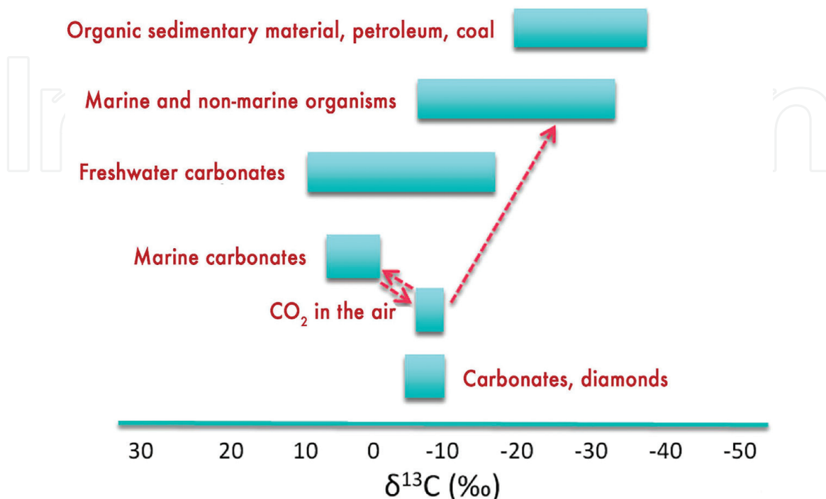
Figure 7. Isotopic fingerprint of naturally occurring carbon.
