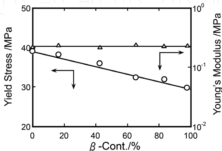
Figure 5. Yield stress and Young's modulus plotted against the \beta -contents for the \beta -nucleated iPP.
