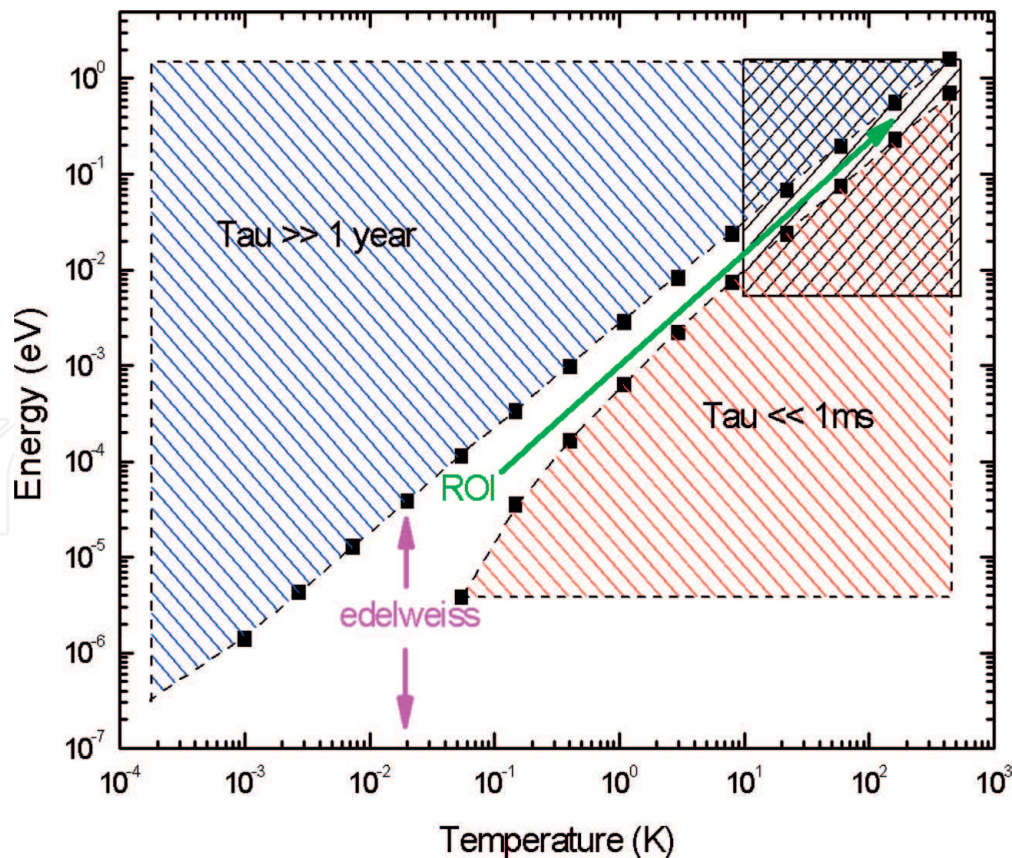
Figure 2. Diagram showing the energy of the trapping level in Ge band gap versus temperature, using a simple Boltzmann factor. This is valid at high temperature for thermal emission with a time constant \tau . The region investigated by DLTS is delimited by the upper square on the right. The purple arrow shows the operation of DM cryogenic experiments such as EDELWEISS.
