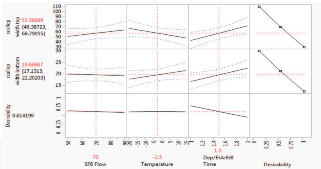
Figure 7. DRIE profile scalloping prediction and desired profiles [23].
