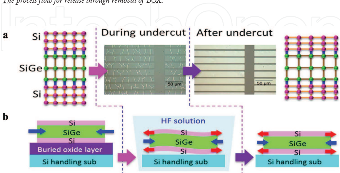
Figure 10. (a) Atomic lattice schematic diagram showing the strain sharing principle. Optical images show the strained NM during release and after finishing release. (b) Process flow to implement the strain sharing principle and the release. Reproduced with permission [25]. Copyright 2013, nature publishing group.
