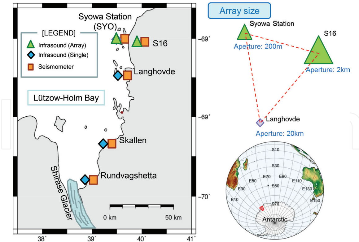
Figure 2. (Left) locations of array deployment in the Lützow-Holm Bay (LHB). Array stations of infrasound (green triangles), single stations of infrasound (blue diamond), and broadband seismometers (orange squares) are shown. (Upper right) Array configuration of infrasound stations so as to localize the source signals. Tripartite arrays have been deployed by small size (at Syowa Station (SYO); aperture of 200 m), medium size (at S16, S17, P50; aperture of 2 km), and large size (combination of other outcrop stations such as Langhovde, aperture of 20 km or larger).
