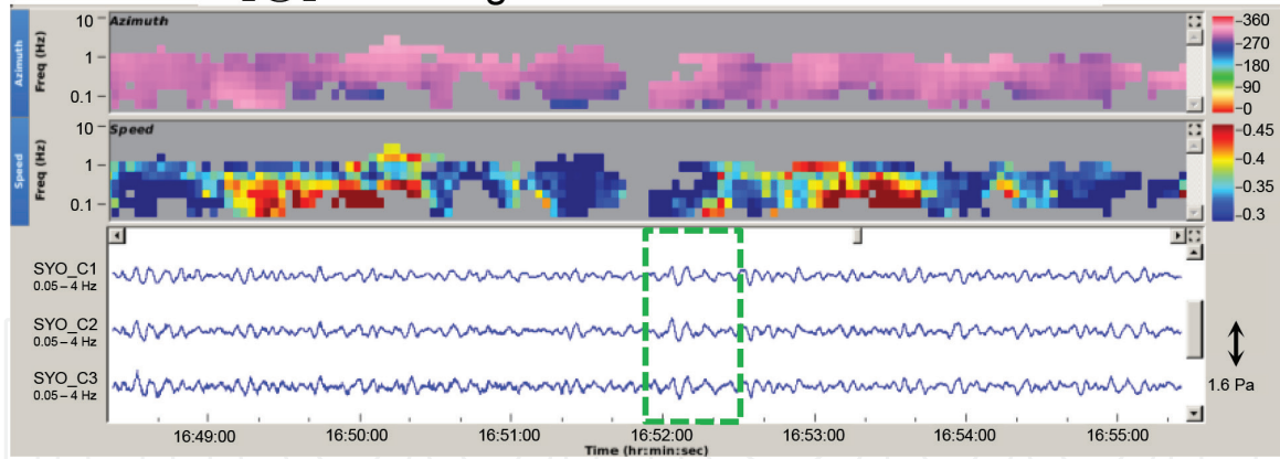
Figure 3. Detection of infrasonic signals associated with discharge events of sea ices from LHB on (1) April 3, 2016 (forecasted origin time, 03:27 UTC), (2) April 11, 2016 (forecasted origin time, 22:00 UTC), and (3) April 7, 2016 (forecasted origin time, 16:42 UTC). The upper panels show the results of PMCC analysis: Back azimuth (station-to-source) direction and the apparent velocities. The lower panels represent band pass-filtered waveforms observed at SYO array. Green broken squares on the waveforms correspond to the time windows of detected infrasonic events.
