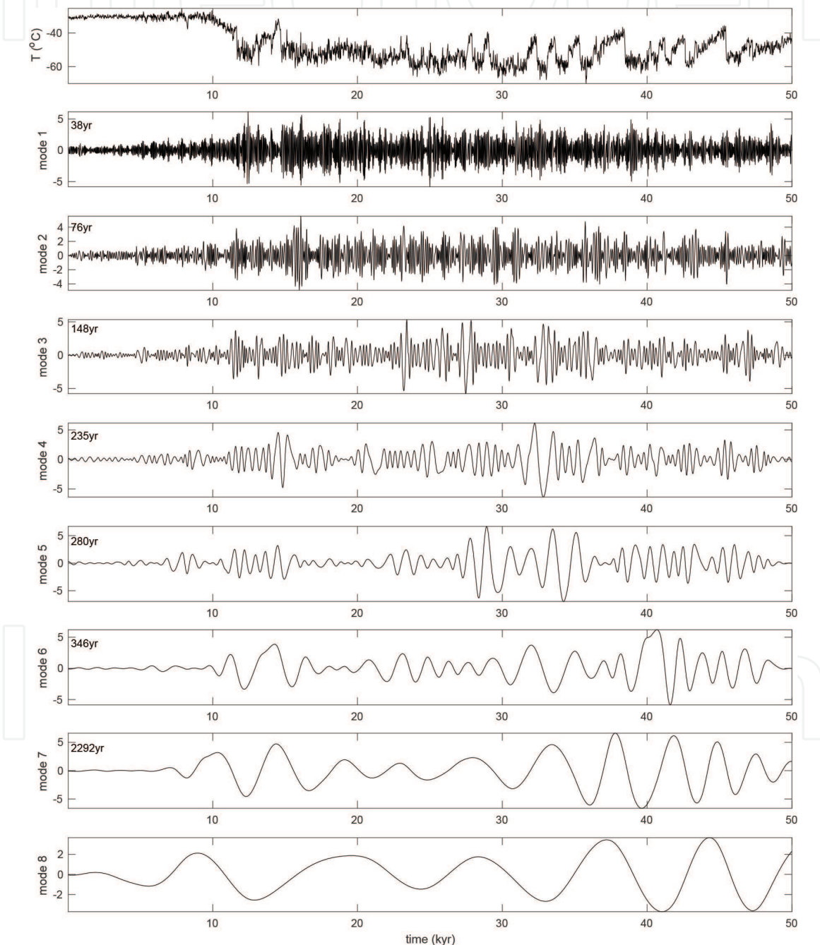
Figure 3. (Upper panel) The air temperature estimated from the GISP2 \Delta^{18}\text{O} data. The evolution of the temperature, which is given at a 20-year cadence, its EMD modes in the relevant frequency range, and the characteristic quasi-periods are shown (see the upper left side of the figure). In accordance with the results for the Na ion shown in Figure 2 , we see that the amplitudes of the variations of temperature were much greater before the Holocene. The warming at the termination of the YD was very abrupt and may have been accomplished in only a single decade at 11,570 \pm 200 ybp [18].
