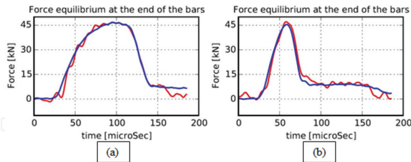
Figure 17. Force equilibrium on the edge of the incident bar (red line) and transmitted bar (blue line) for PPSGFC under (a) 558.5 \text{ s}^{-1} and (b) 891.1 \text{ s}^{-1} .
