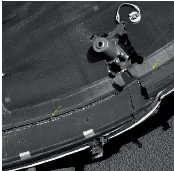
Figure 14. Evidence of fresh blueberries collected by heat shield. Image 1P158281536EFF40C2P2368L6M1 (sol 339). Image courtesy: NASA/JPL & M Lyle.
