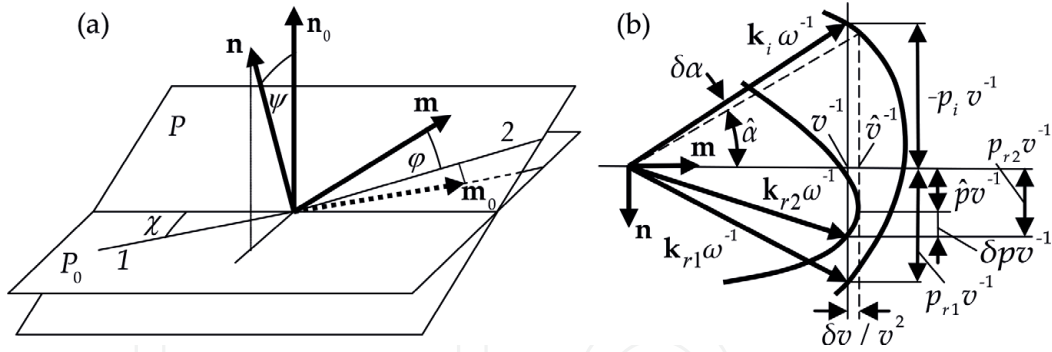
Figure 2. (a) Perturbations of the crystal surface P_0 \rightarrow P , its normal orientation n_0 \rightarrow n and the propagation direction m_0 \rightarrow m ; (b) the scheme of the resonance reflection (only outer and middle sheets of the slowness surface are shown).
