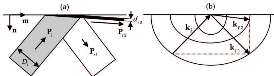
Figure 1. Scheme of excitation of a narrow beam near total internal reflection in the \mathbf{r} space (a) and \mathbf{k} space (b) with P_i , \mathbf{k}_i ; P_{r1} , \mathbf{k}_{r1} ; and P_{r2} , \mathbf{k}_{r2} to be mean Poynting and wave vectors of the incident, parasitic, and excited beams, respectively.
