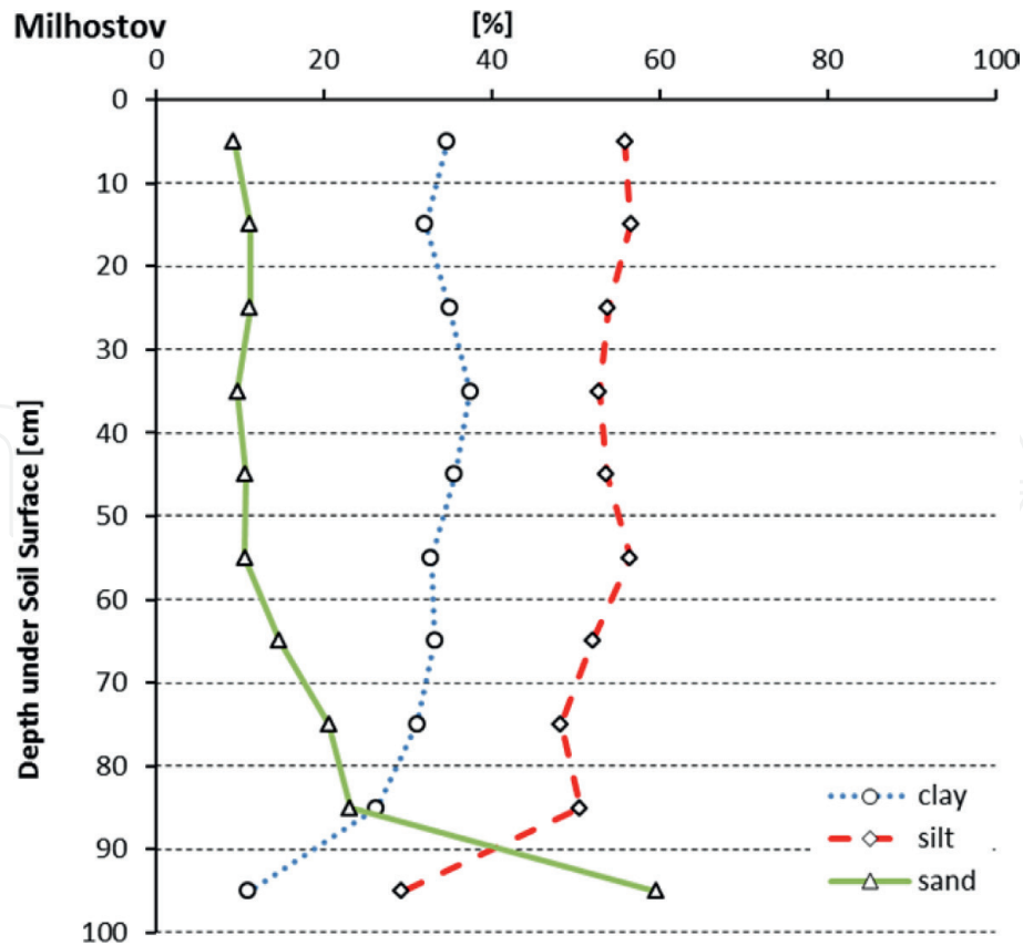
Figure 2. Content of clay, silt and sand to the soil profile vertical to 1 m depth.
