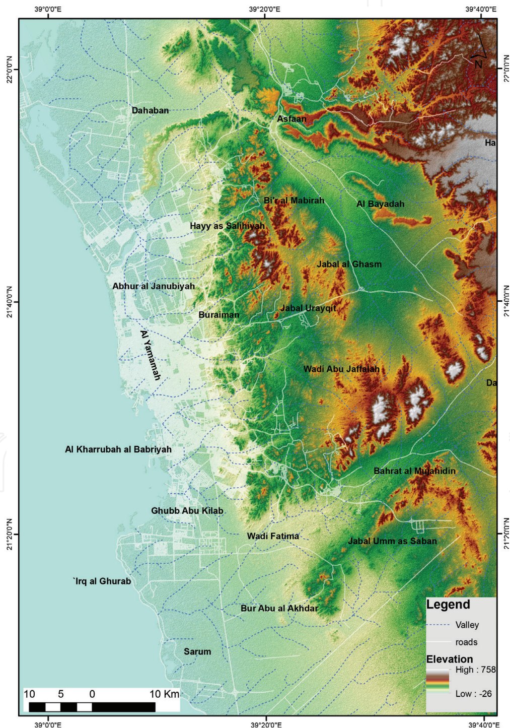
Figure 4. Geomorphological and topographic contexts of Jeddah city.
