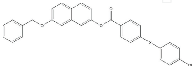
23, X = \text{---N=N---} , R = \text{---C}_n\text{H}_{2n+1} , n = 6–10
