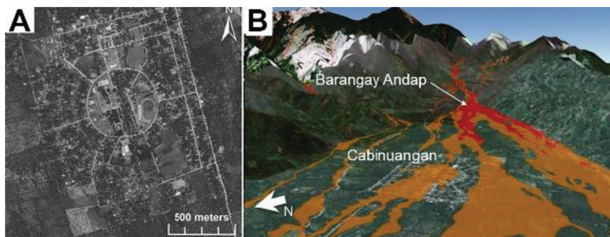
Figure 2. New Bataan. A= Andap, Google image of Cabinuangan (the central district of New Bataan) before the debris flow. B= Southward facing three-dimensional terrain diagram of Andap and Cabinuanga after the Mayo River disaster. Red areas are boulder-rich "true debris flow; orange areas are deposits of more dilute "hyperconcentrated" flows.
