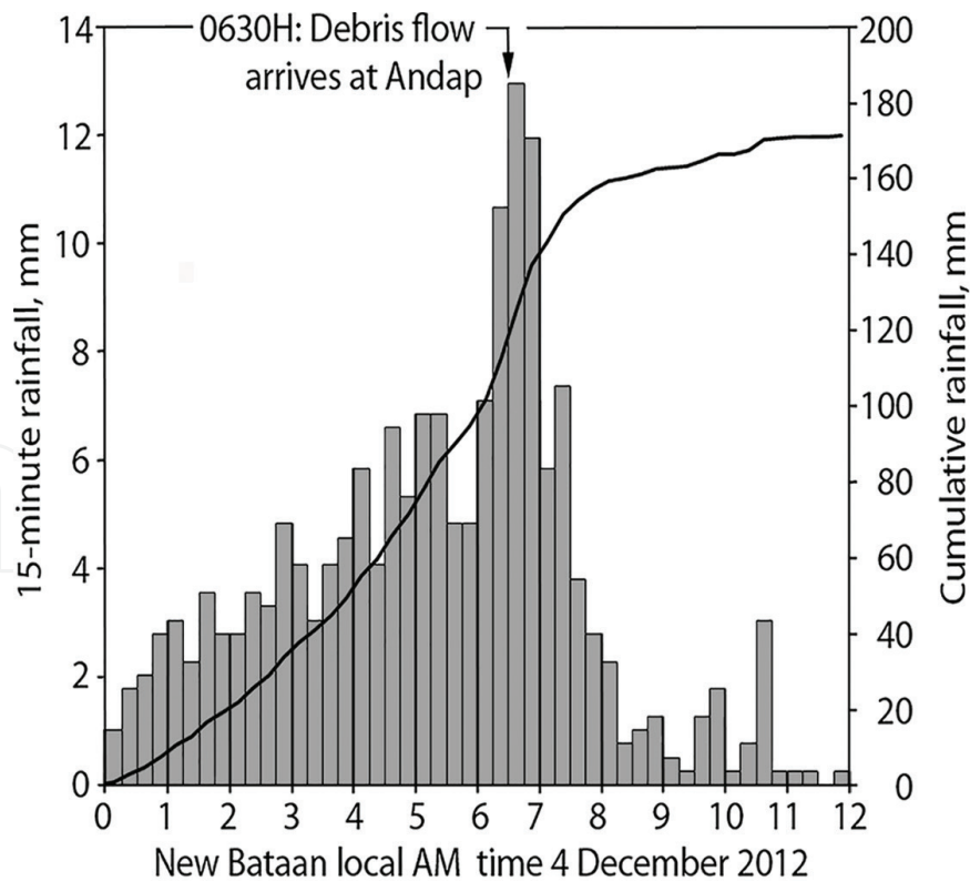
Figure 5. The rainfall that triggered and sustained the Mayo debris flow. Histogram measures the rain that fell during successive 15-minute intervals; 120 mm had accumulated by the time the debris flow hit Andap. Another 24 mm of peak rainfall sustained the flow until 0700H before the storm began to wane.
