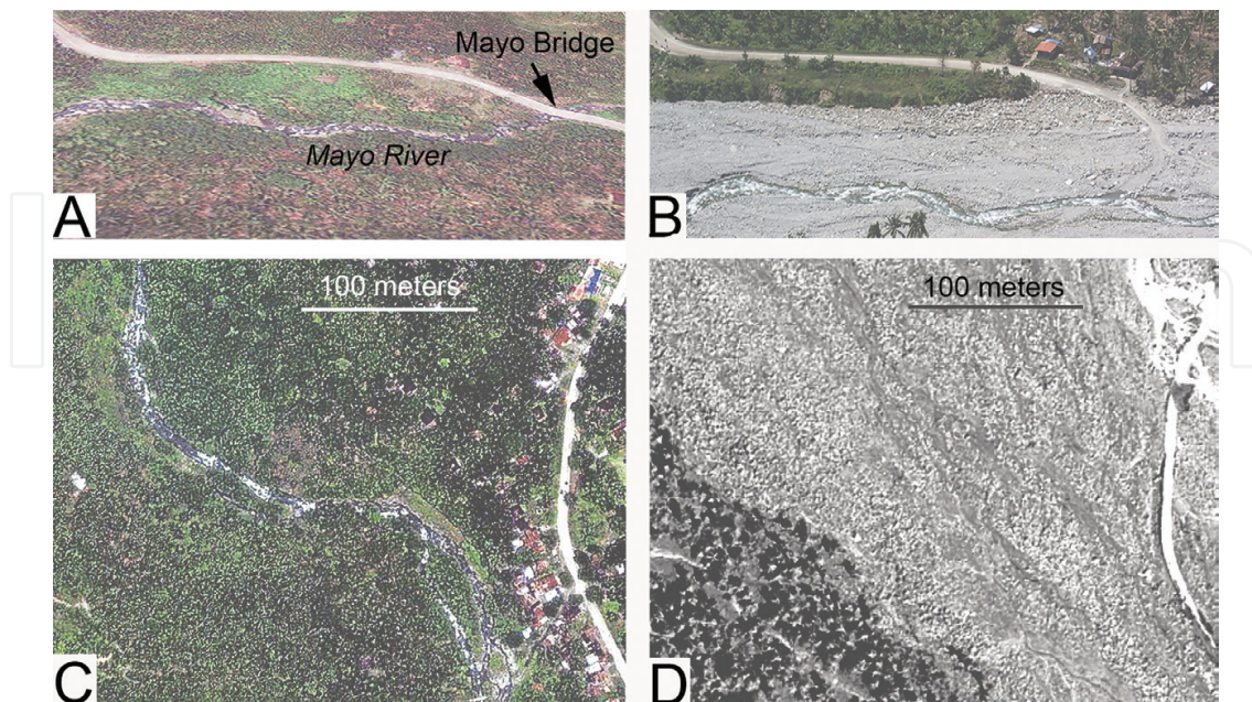
Figure 8. Upstream impacts of the debris flow. (A) Google image of the Mayo River and Mayo Bridge before the debris flow. (B) Post-Bopha air photo of the same area. The large boulder in Figure 3C is where the temporary road crosses the stream. (C) Air photo of Andap before Bopha. (D) Same area after the debris flow.
