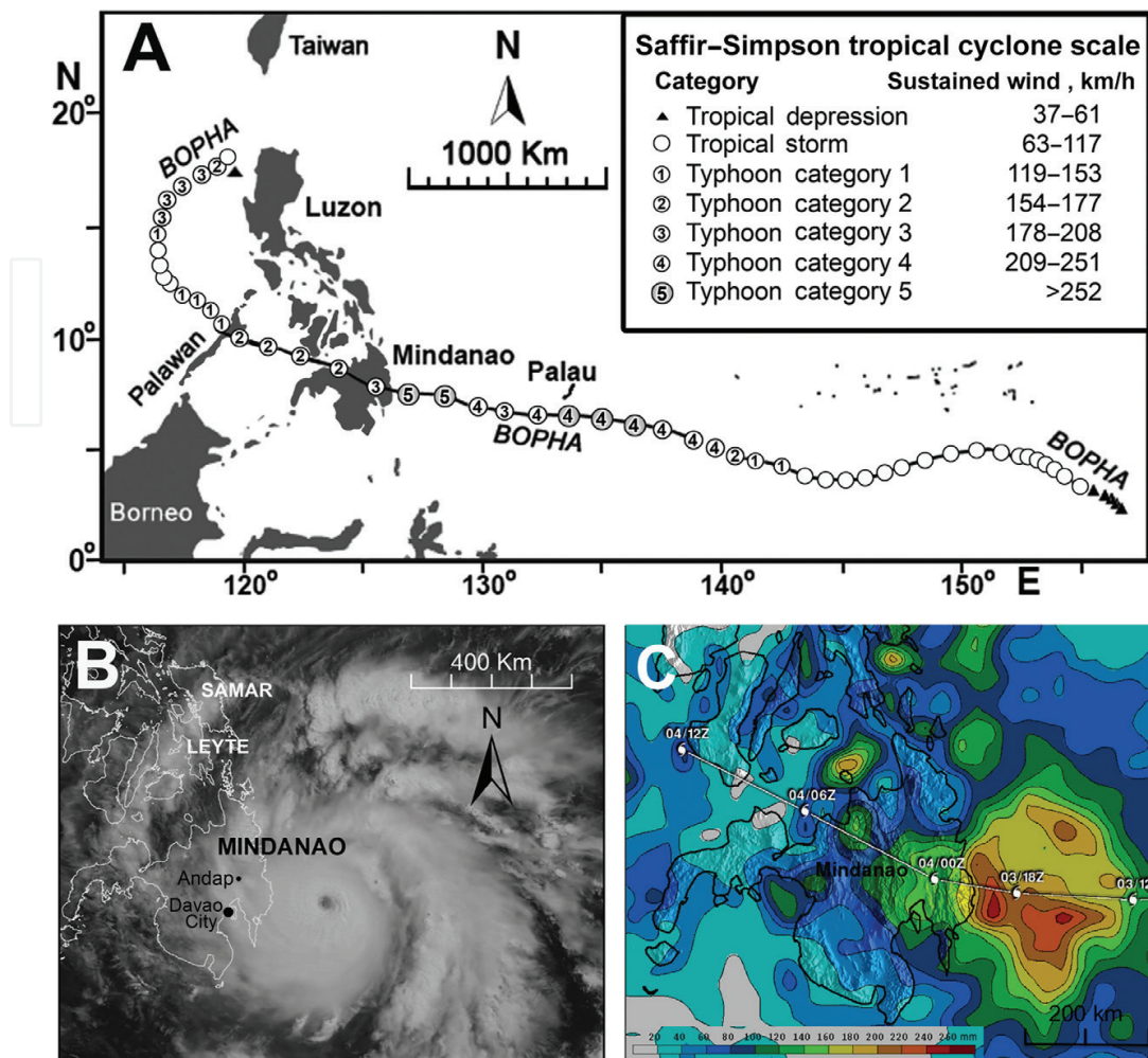
Figure 4. Typhoon Bopha (Pablo). (A) Track and development of the Super Typhoon. New Bataan, Andap, and the Maragusan rain gauge lie beneath the Category 3 icon following the Mindanao landfall. (B) Bopha nearing landfall (modified from [28]). (C) Tropical Rainfall Measurement Mission (TRMM) image from which NASA [28] estimated that Bopha delivered over 240 mm of rainfall near the coast.
