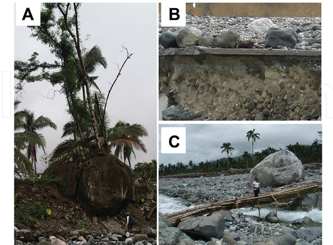
Figure 3. Debris-flow deposits in the New Bataan area. (A) Boulder in ancient reverse-graded debris-flow deposit. Well-established trees indicate an age of some decades prior to the settlement of the town. (B) Old debris-flow deposits underlying New Bataan—Andap high-way. Boulders and cobbles are separated from each other by a matrix of finer-grained sediment, as they were while still flowing. For scale, the concrete is 15-cm thick. The coarse sediments atop the highway are new debris-flow deposits from Typhoon Bopha. (C) Boulder-rich deposits of debris flows that destroyed much of the barangay, at the site of the destroyed Mayo River bridge.
