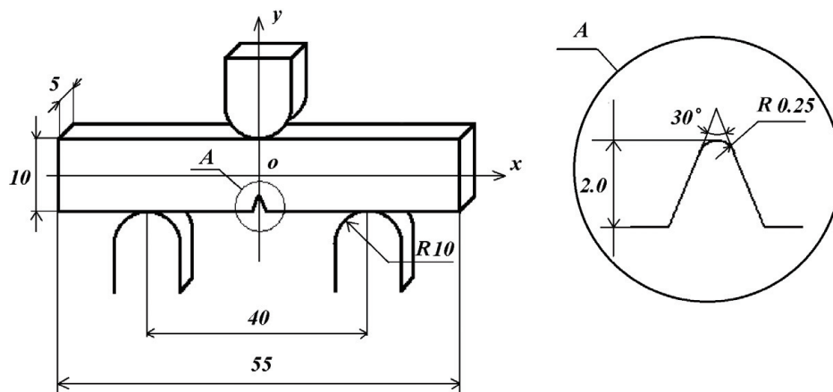
Figure 6. Shape and dimensions of the specimen.
