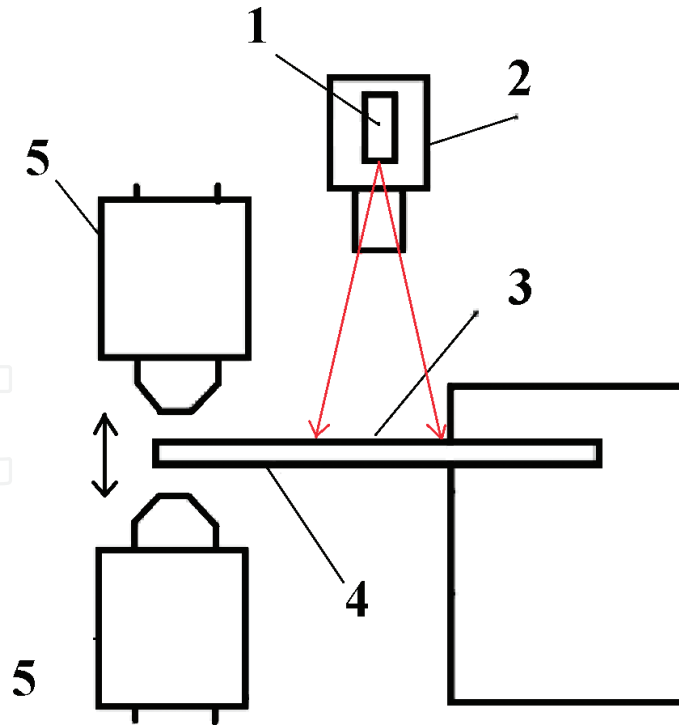
Figure 3. Scheme of periodic bending: 1—laser module, 2—TV camera, 3—control zone, 4—specimen, and 5—electromagnet.
