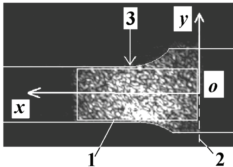
Figure 4. Dimensions and shape of the specimen (top) and speckle pattern (bottom): 1—control zone, 2—clamp line, and 3—maximum stress spot.
